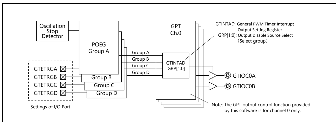
Figure 2.9 Outline of the Relationship Between POEG and GPT (General PWM Timer)
