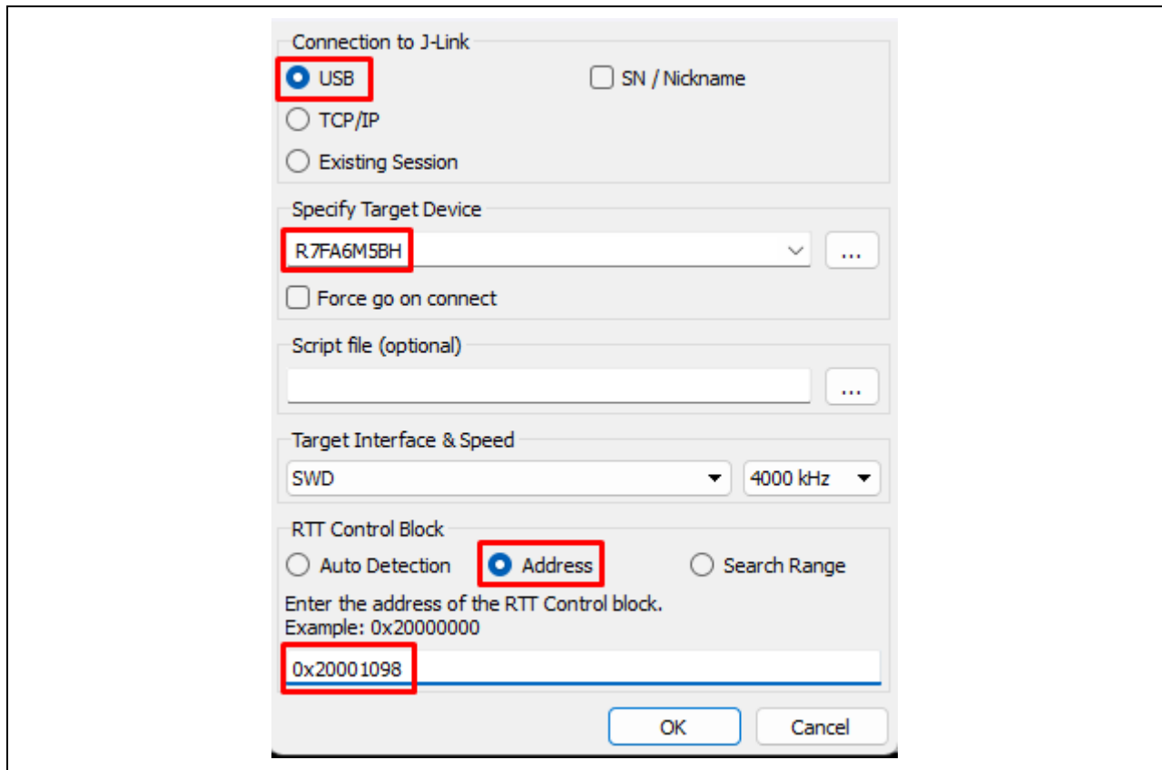
Figure 8. Connect to SEGGER RTT Viewer
