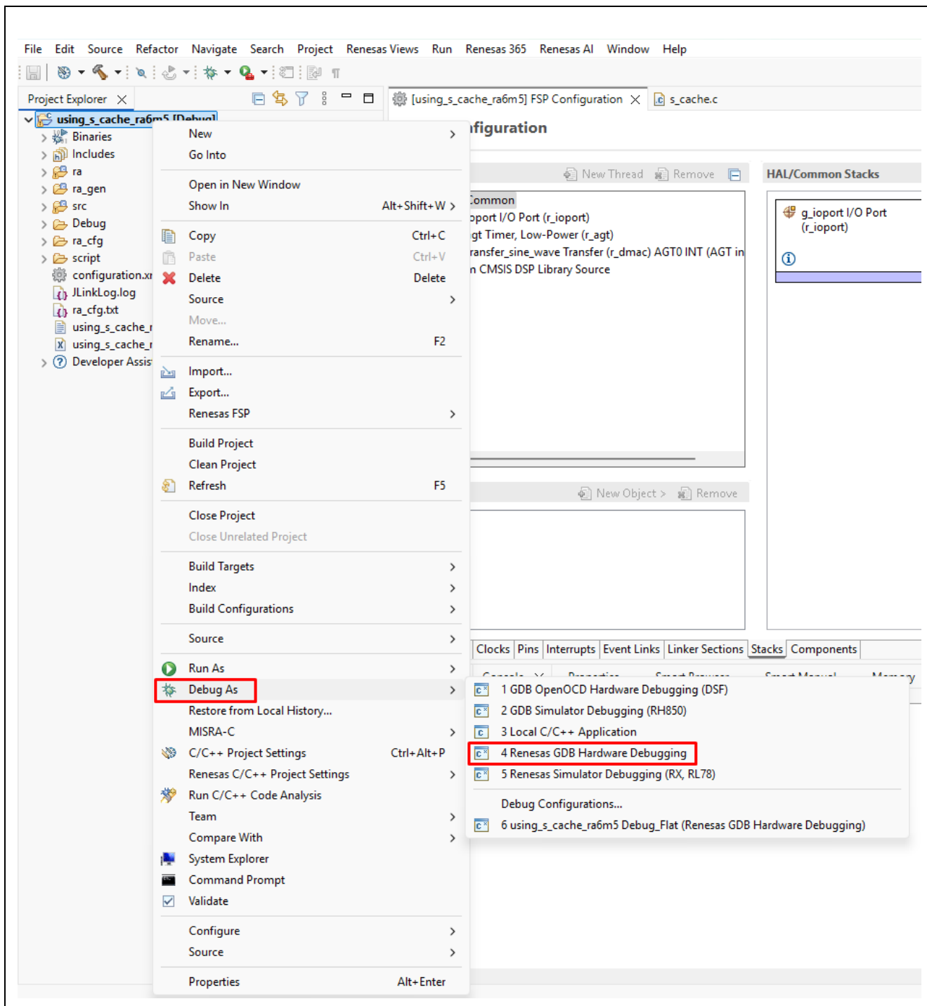
Figure 7. Using S Cache Example Project
