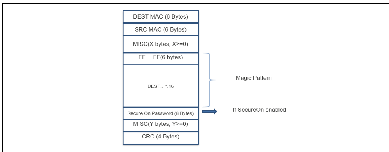
Figure 18. WOL Magic Pattern
