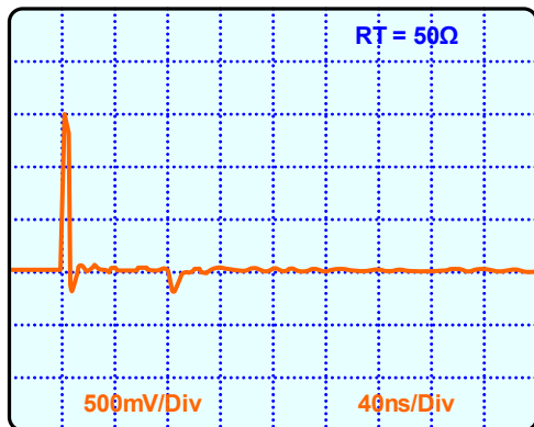
Figure 5. Reflection - Under-Terminated Cable End
