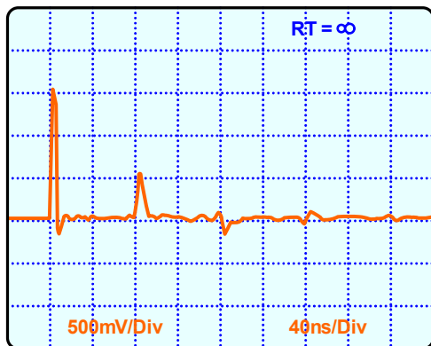
Figure 3. Reflection - Open Cable End
