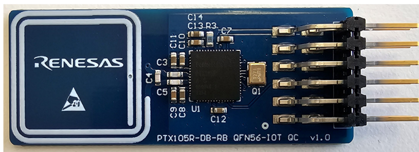
Figure 14. PTX105RQC PMOD Board
