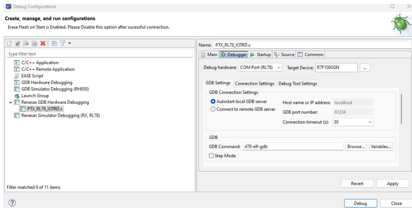
Figure 6. Debug Configurations
