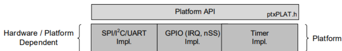
Figure 12. Platform Layer
