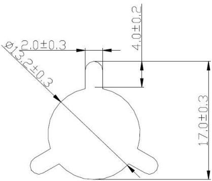
detail AA
