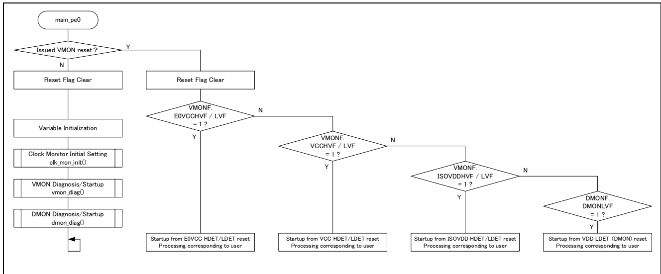
Figure 3-2 Flowchart
