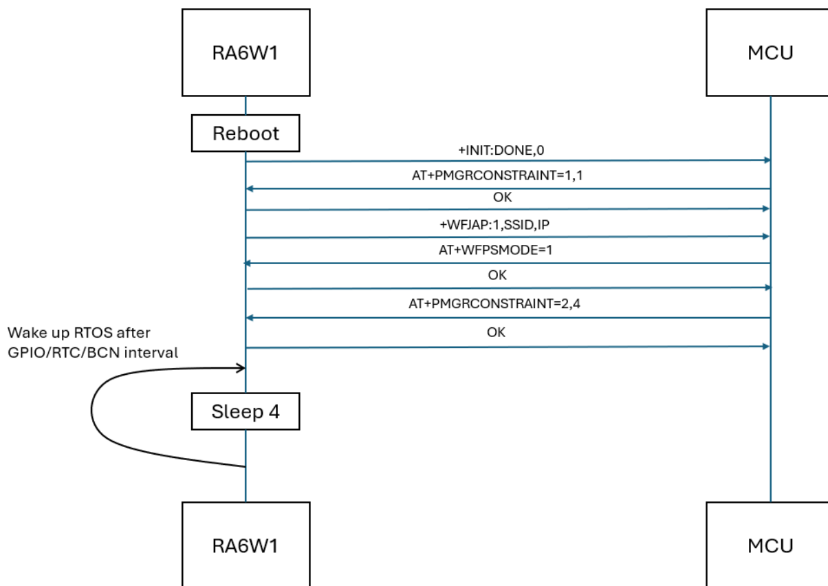
Figure 18. Using AT Command
