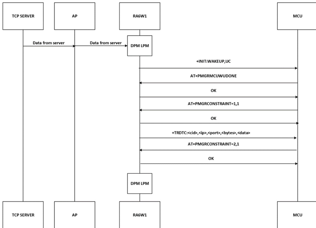
Figure 28. TCP client receive flow using AT commands
