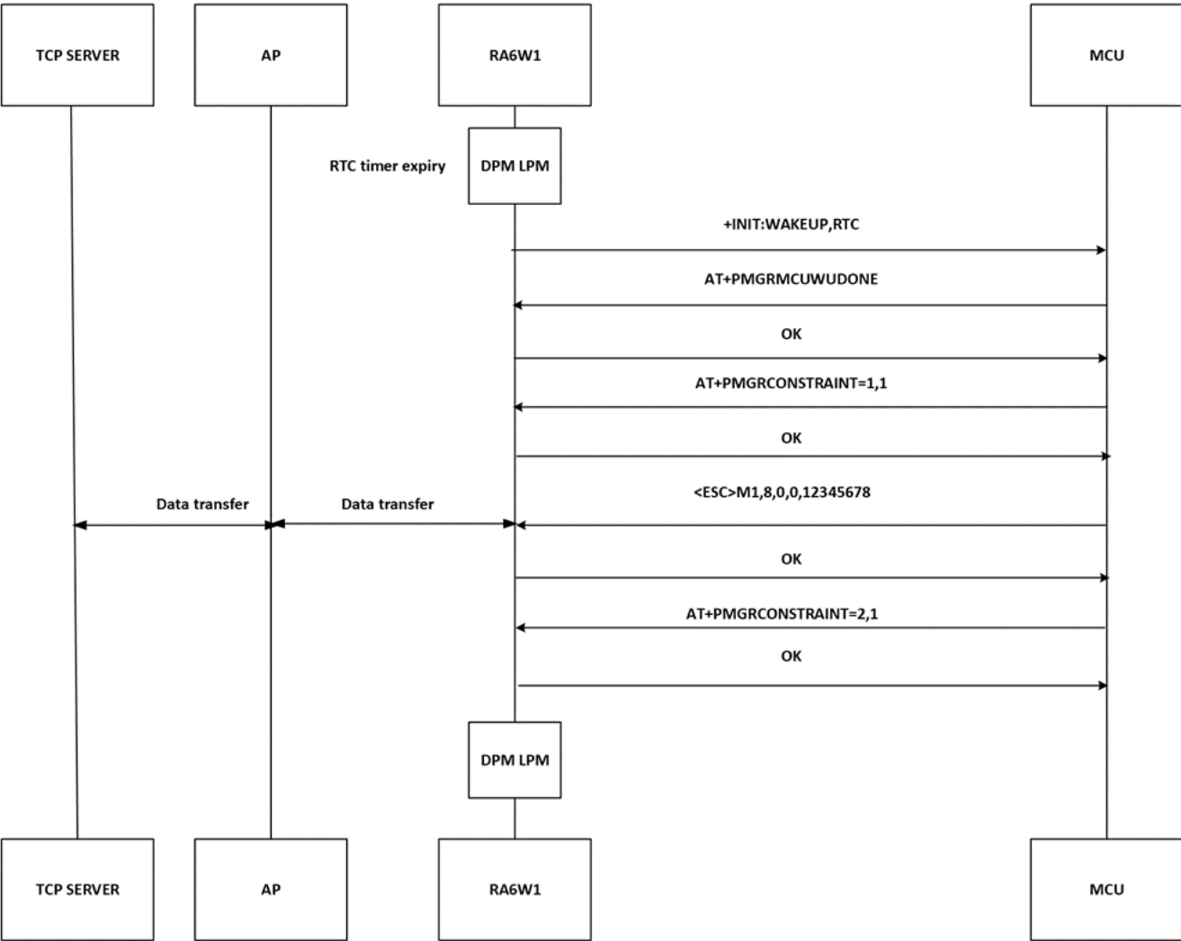
Figure 27. TCP client send flow using AT commands
