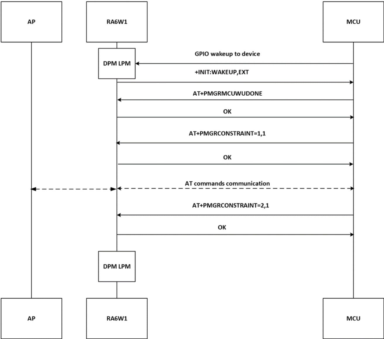
Figure 21. Flow of AT commands for waking up by GPIO of MCU
