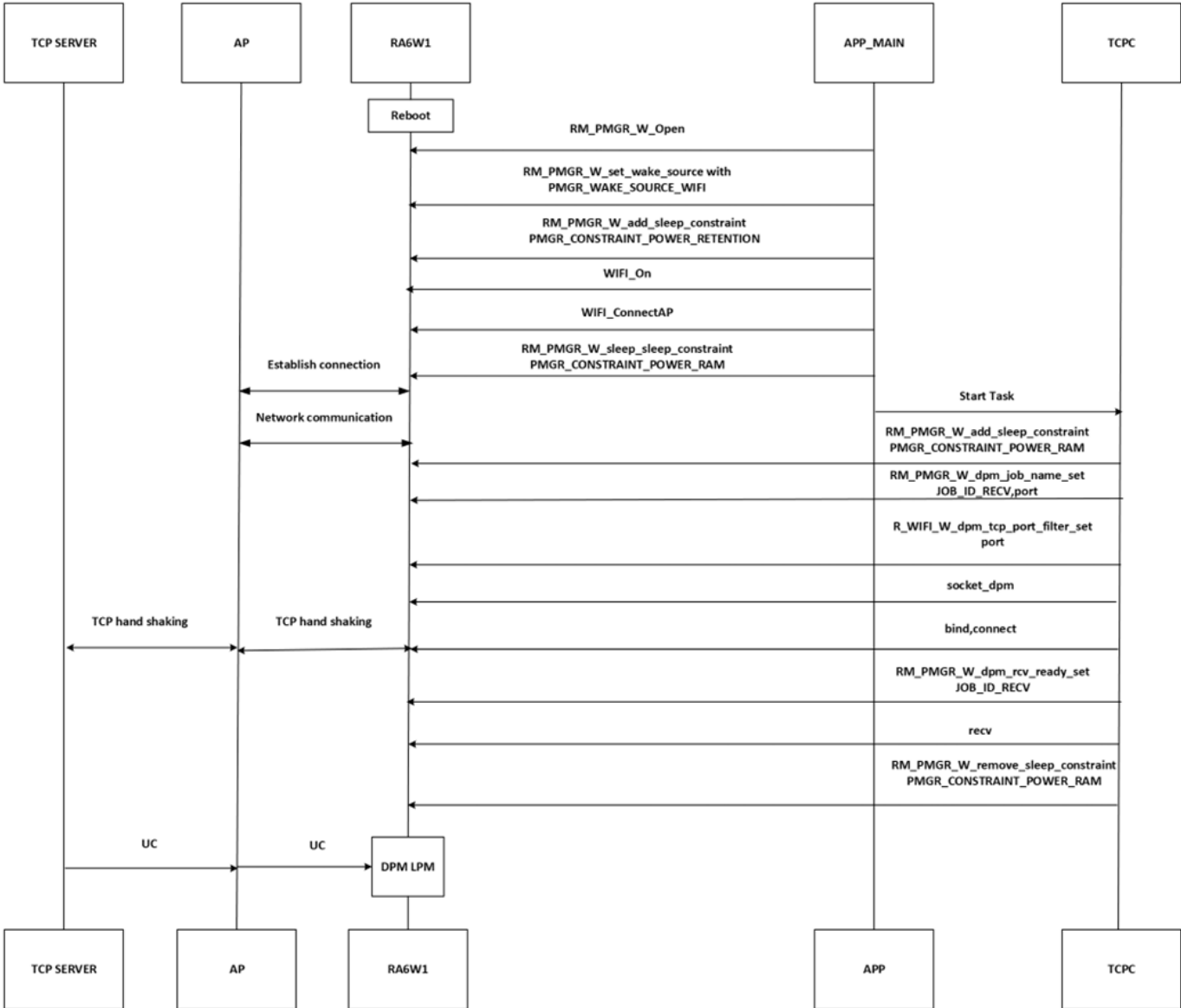
Figure 25. TCP client receive function using API
