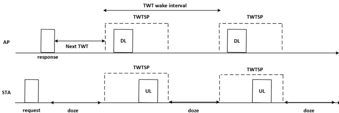
Figure 5. TWT basic flow
