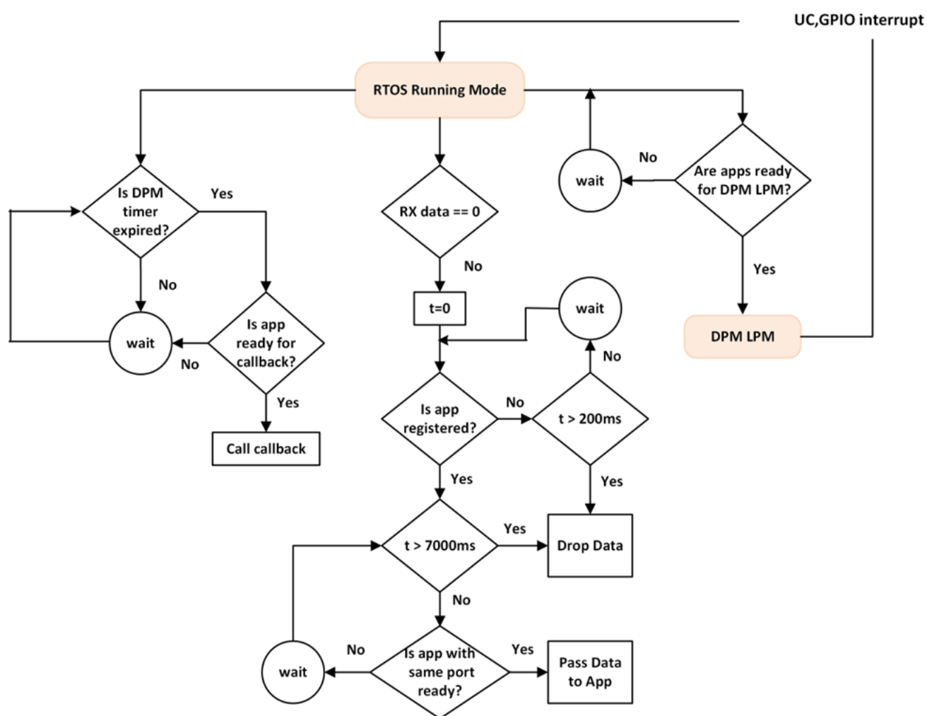
Figure 6. DPM service in RTOS running mode
