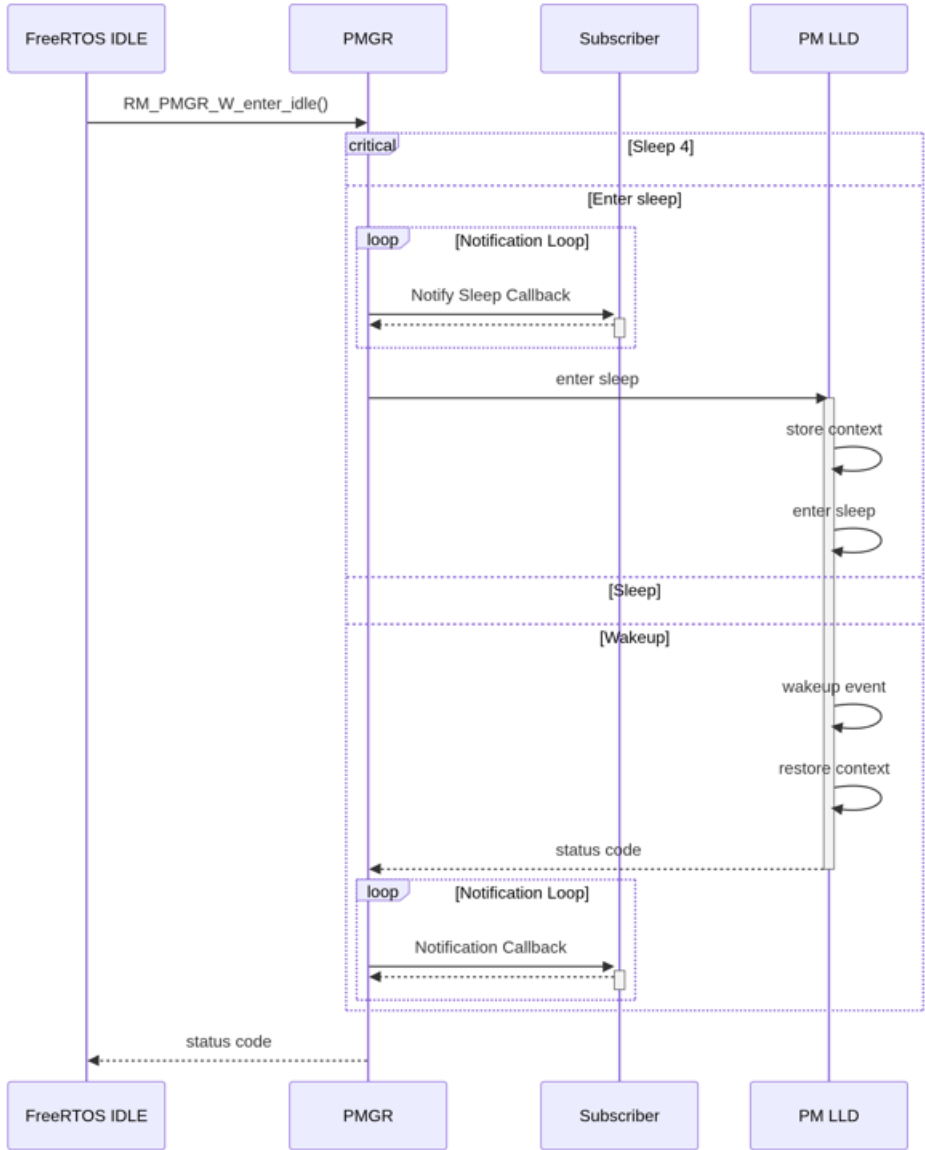
Figure 20. Sleep 4 Enter/Exit Sequence
