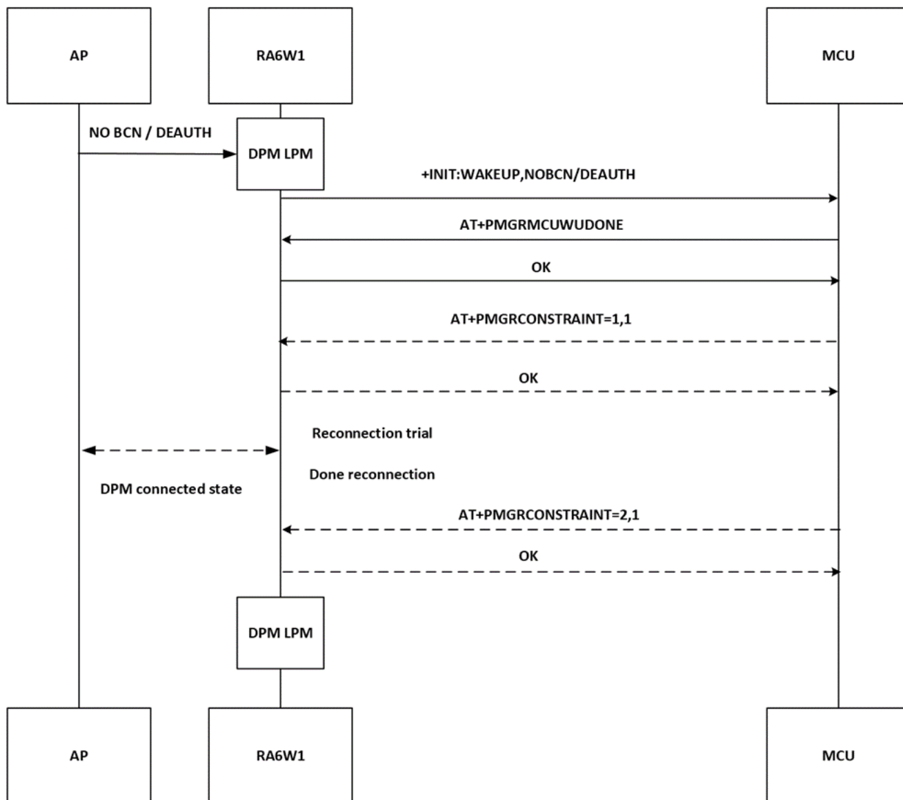
Figure 23. Flow of AT commands for waking up by disconnection from AP
