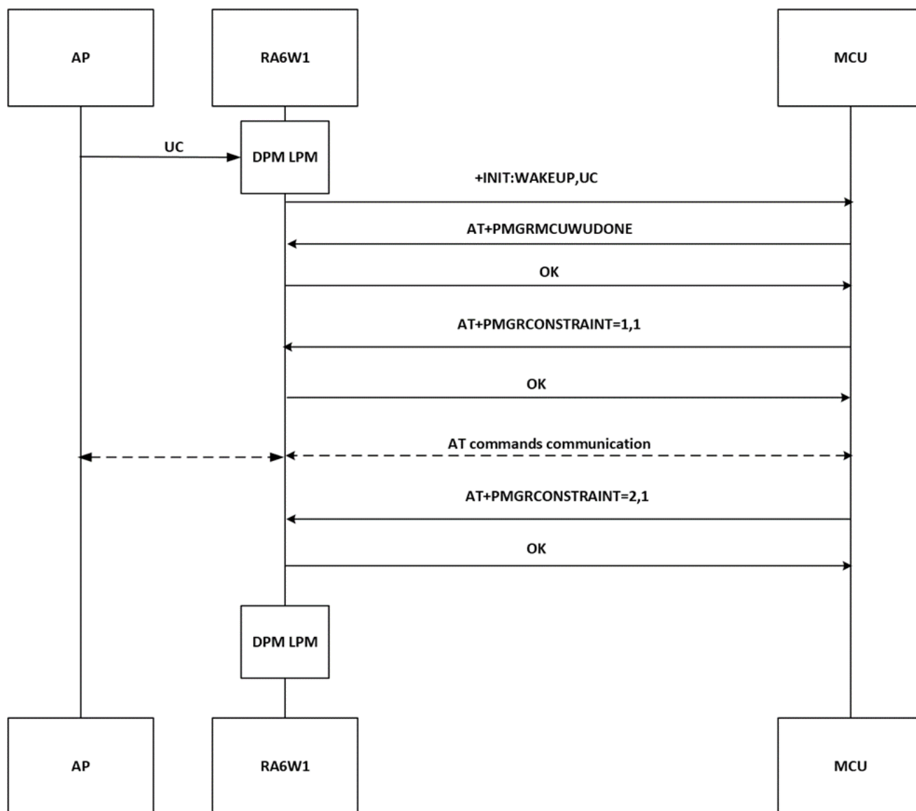
Figure 22. Flow of AT commands for waking up by UC from AP
