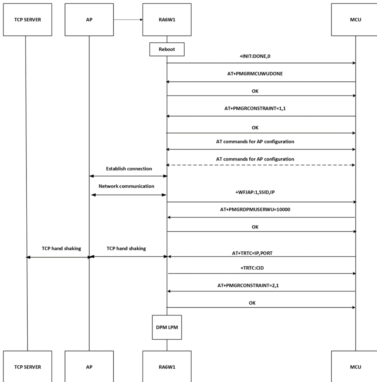
Figure 26. TCP client configuration on DPM
