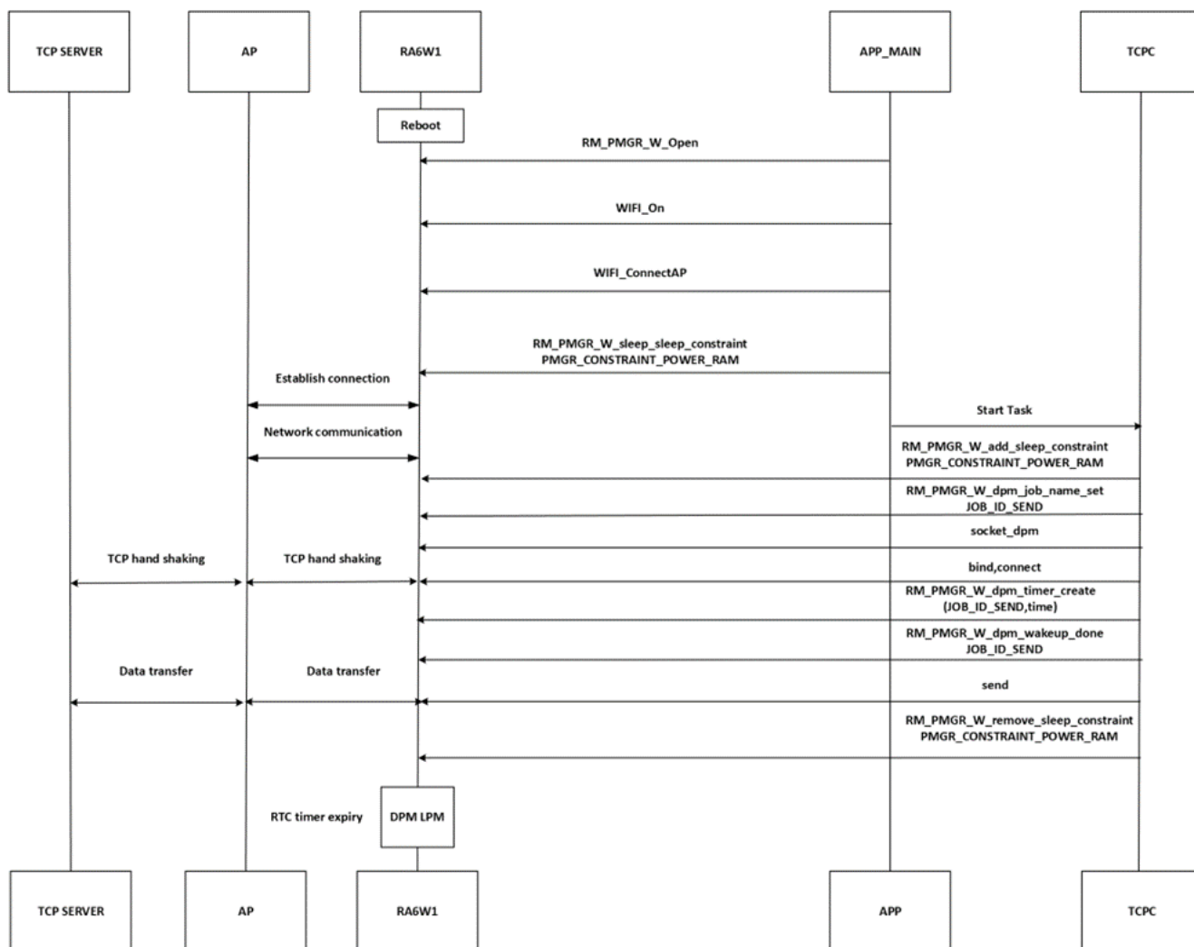
Figure 24. TCP client send function using API
