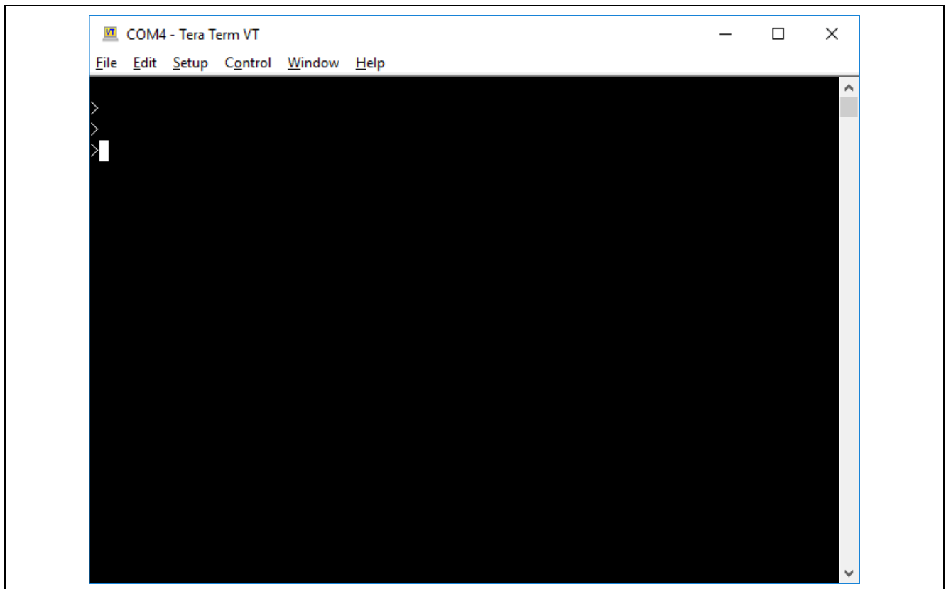
Figure 2.13 Main Window
