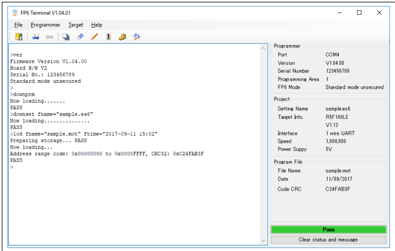
Figure 2.11 Executing Commands
