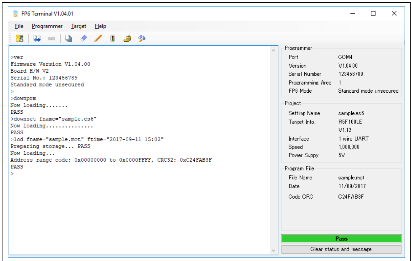
Figure 2.10 Downloading
