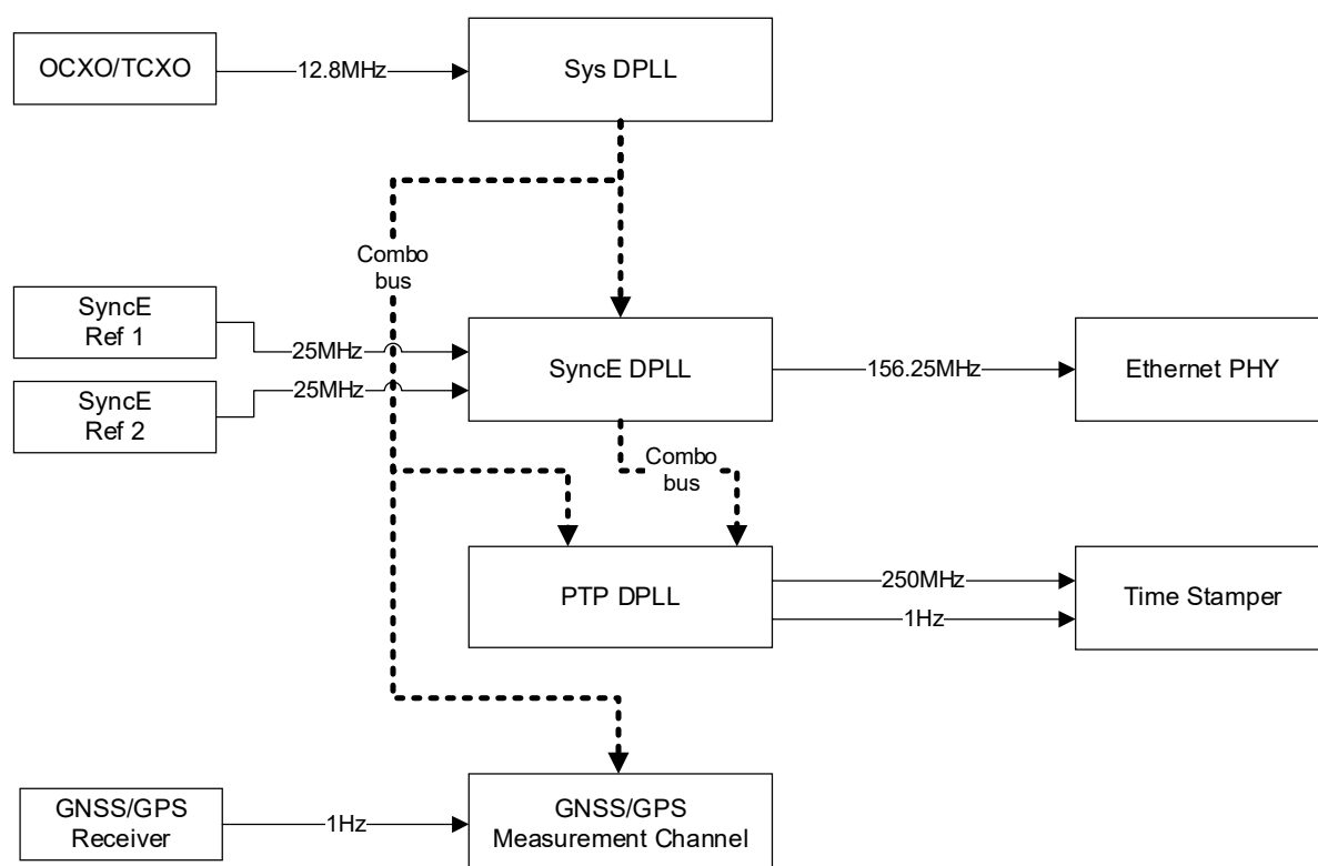
Figure 2. ClockMatrix Simplified Block Diagram
