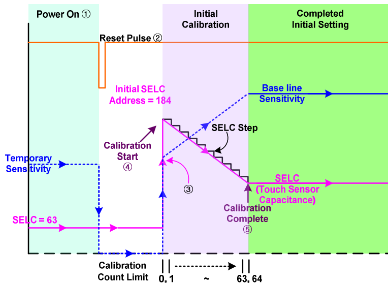
Figure 11: Initial Calibration.
