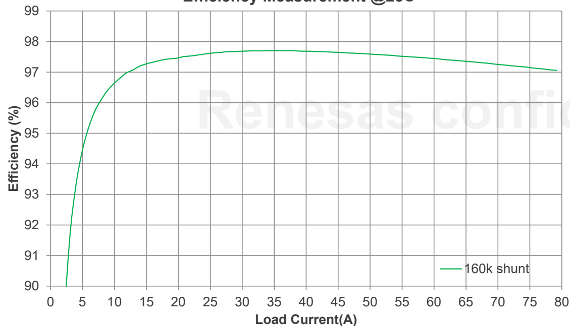
Efficiency Measurement @25C
