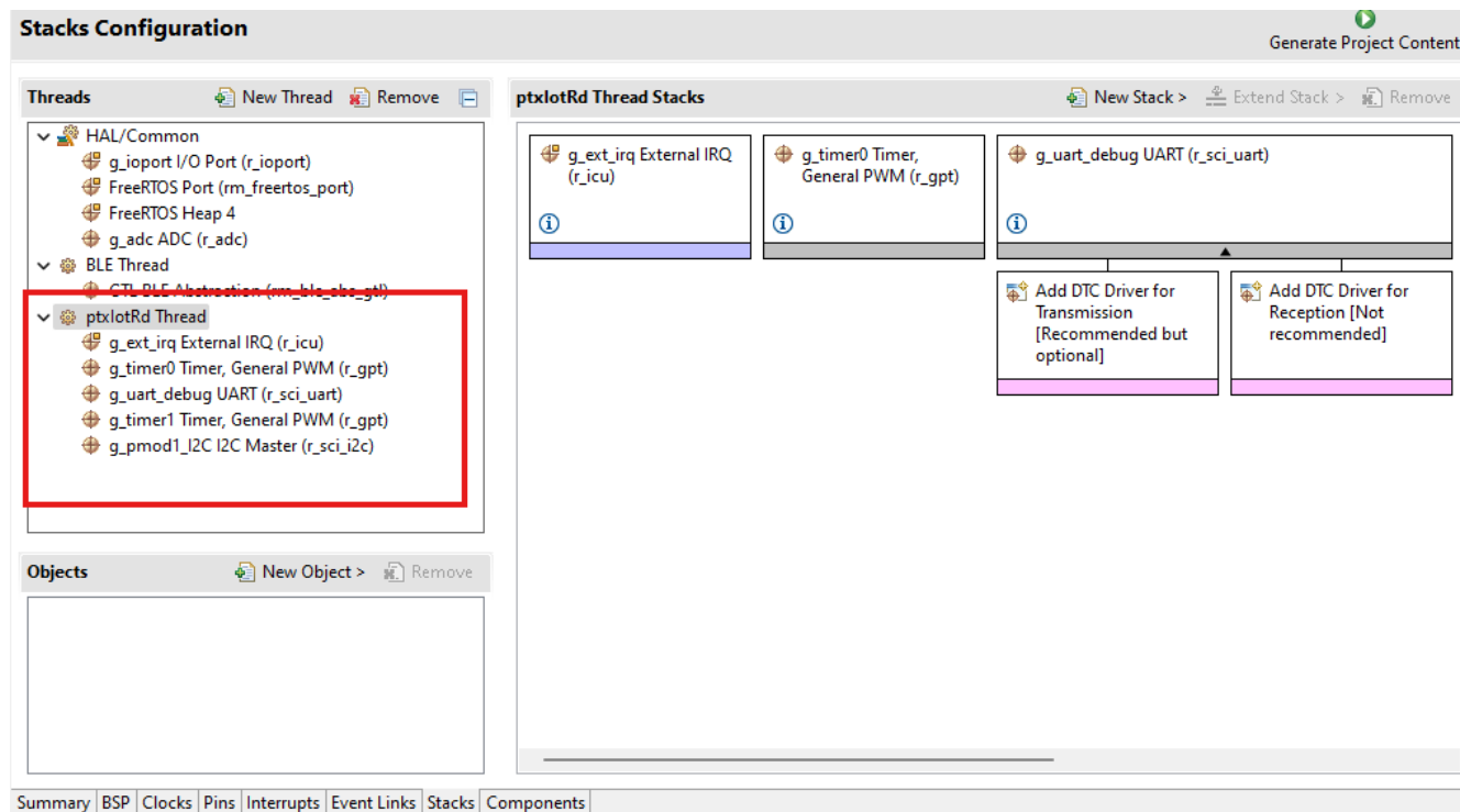
Figure 6. IoT Reader Stacks Configuration
