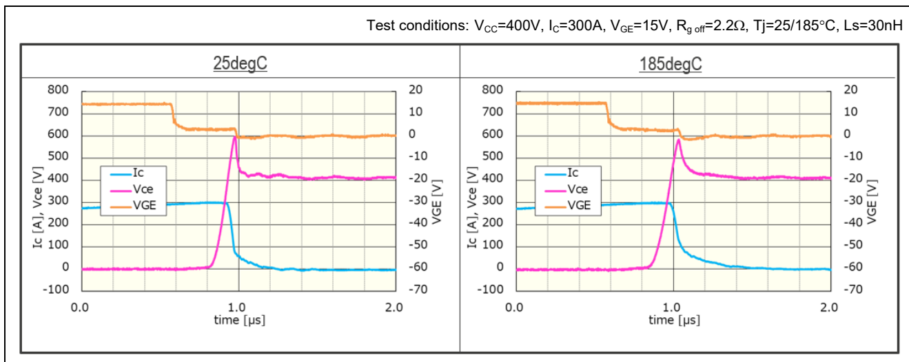
Figure 3-2 Turn-off Waveform (AE5)
