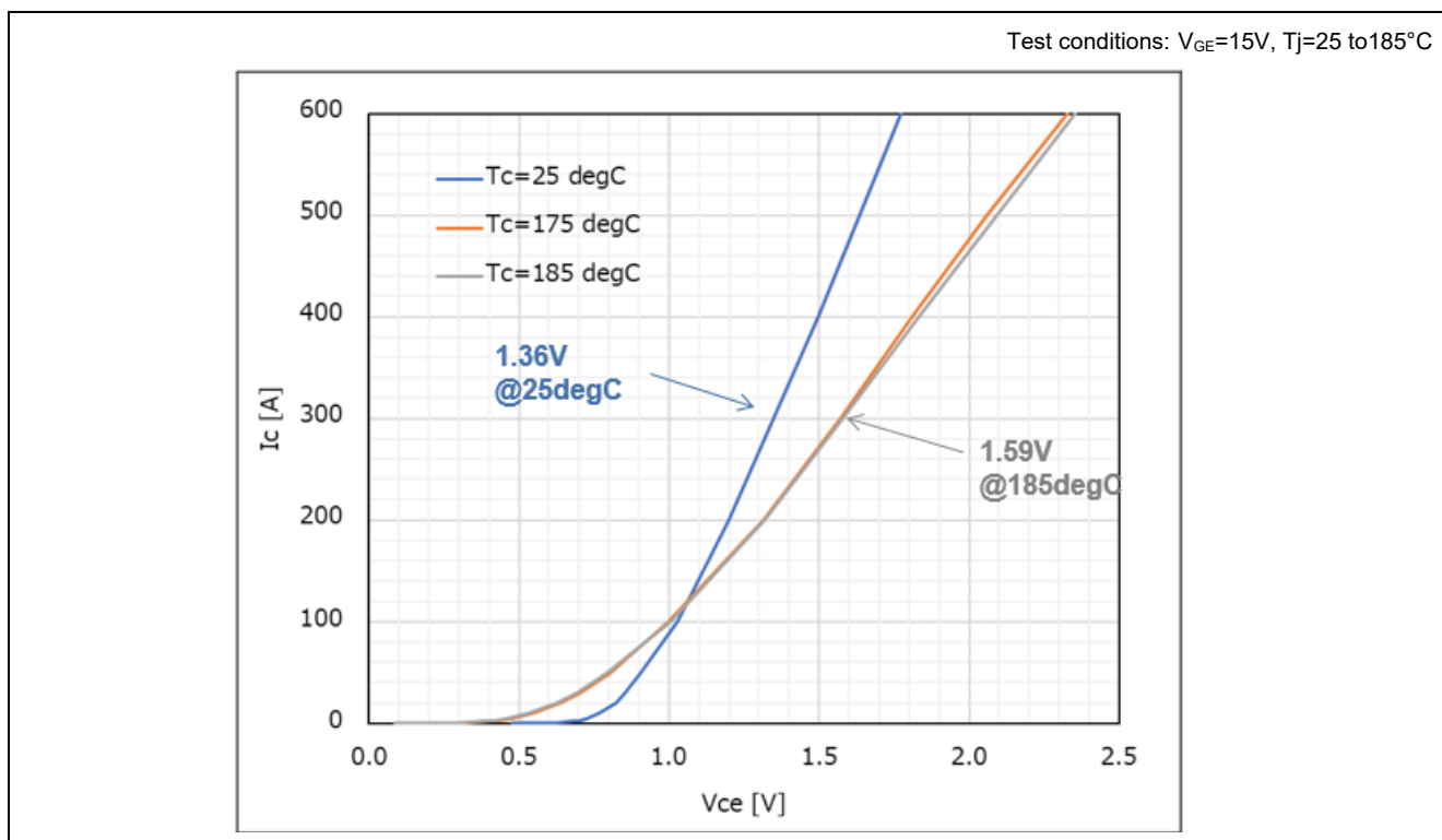
Figure 3-1 V_{CE} - I_C Characteristics (AE5)
