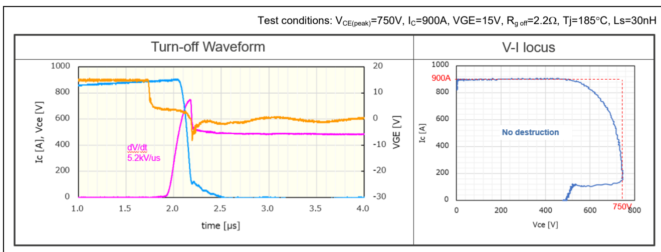
Figure 3-4 RBSOA (AE5)
