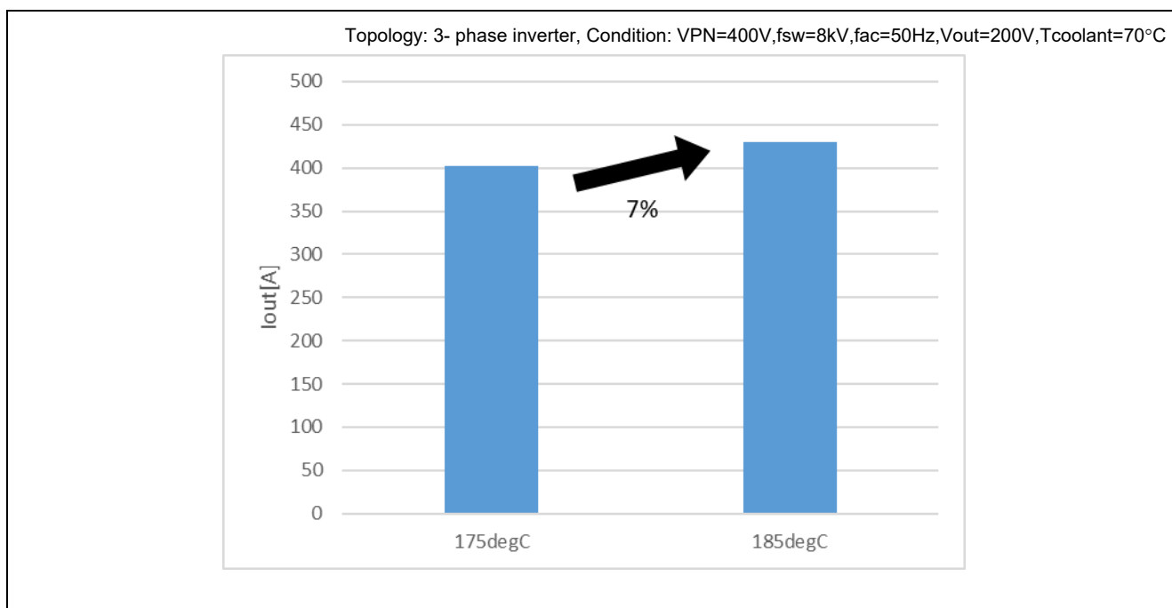
Figure 1-1 Output Current Value During Inverter Operations (AE5 175^{\circ}\text{C} vs. 185^{\circ}\text{C} )
