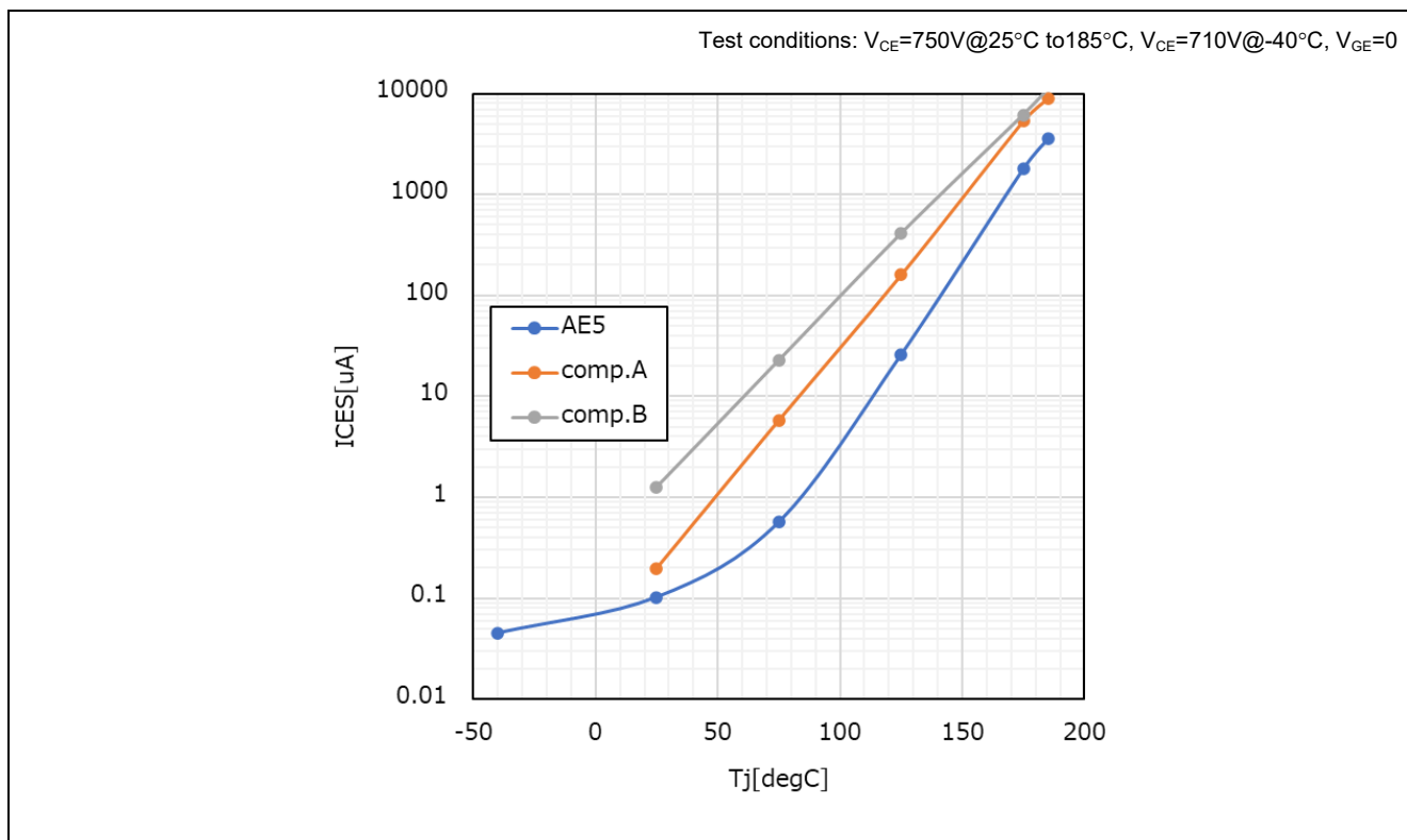
Figure 2-1 I_{CES} - T_j (Renesas IGBT AE5 vs. Competitors)
