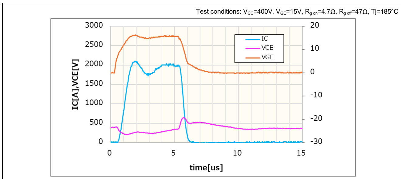
Figure 3-5 Short-circuit Waveform (AE5)
