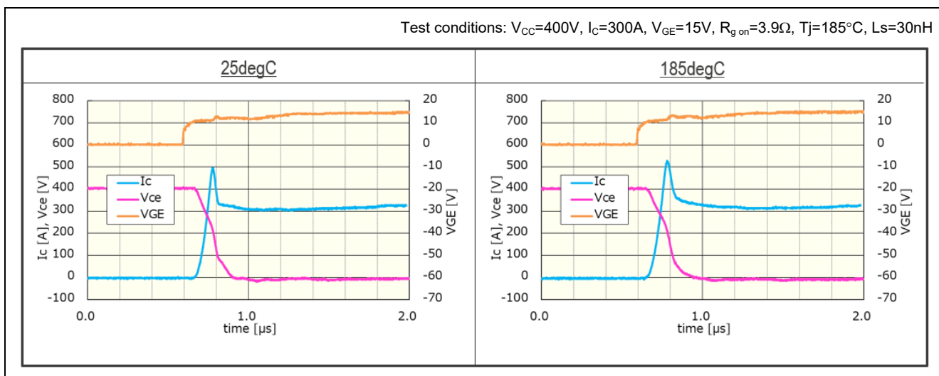
Figure 3-3 Turn-on Waveform (AE5)
