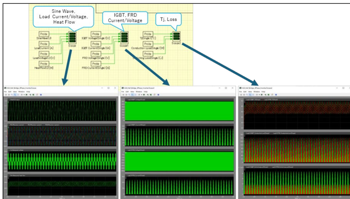
Figure 2-5 Waveform Results
