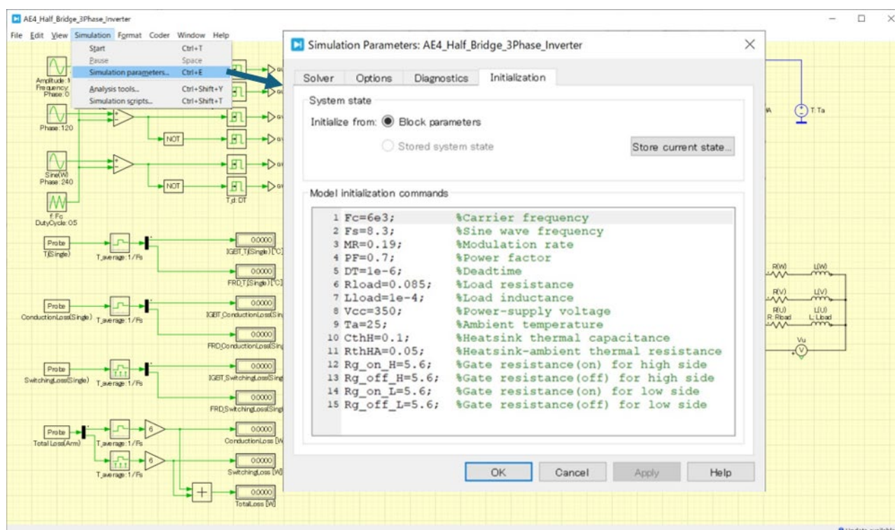
Figure 2-2 Simulation Parameters
