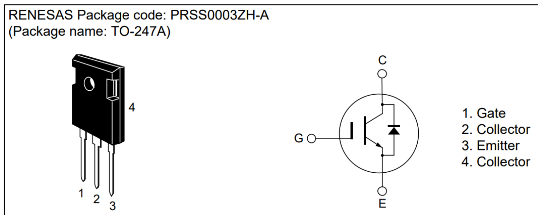
Figure 2-2 RBN50H65T1FPQ IGBT Outline
