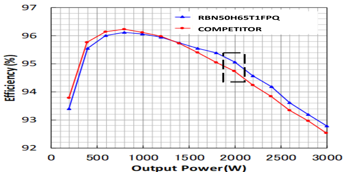
Figure 3-2 Output Power versus Efficiency Change
