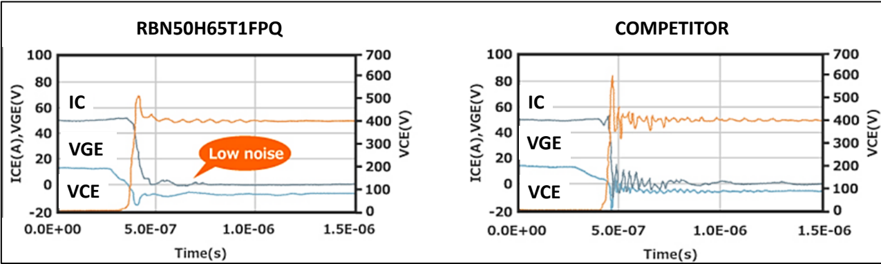
Figure 3-4 Noise Characteristic Comparison
