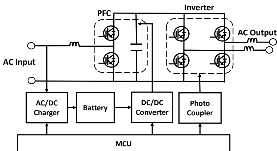
Figure 1-1 UPS Inverter Working principle
