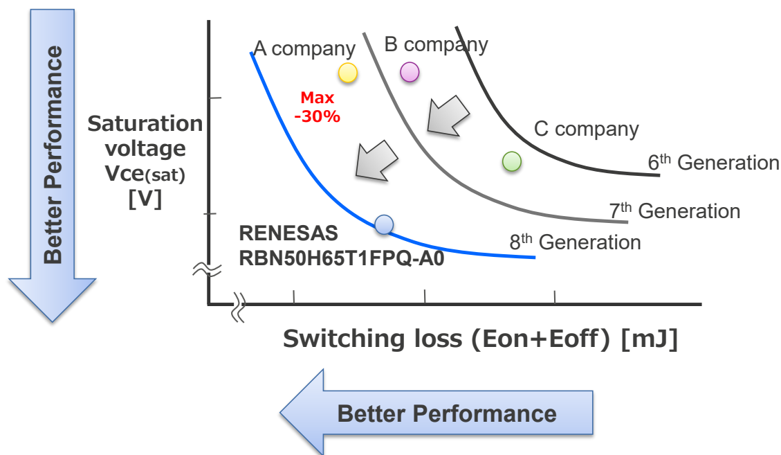
Figure 2-1 IGBT Trend
