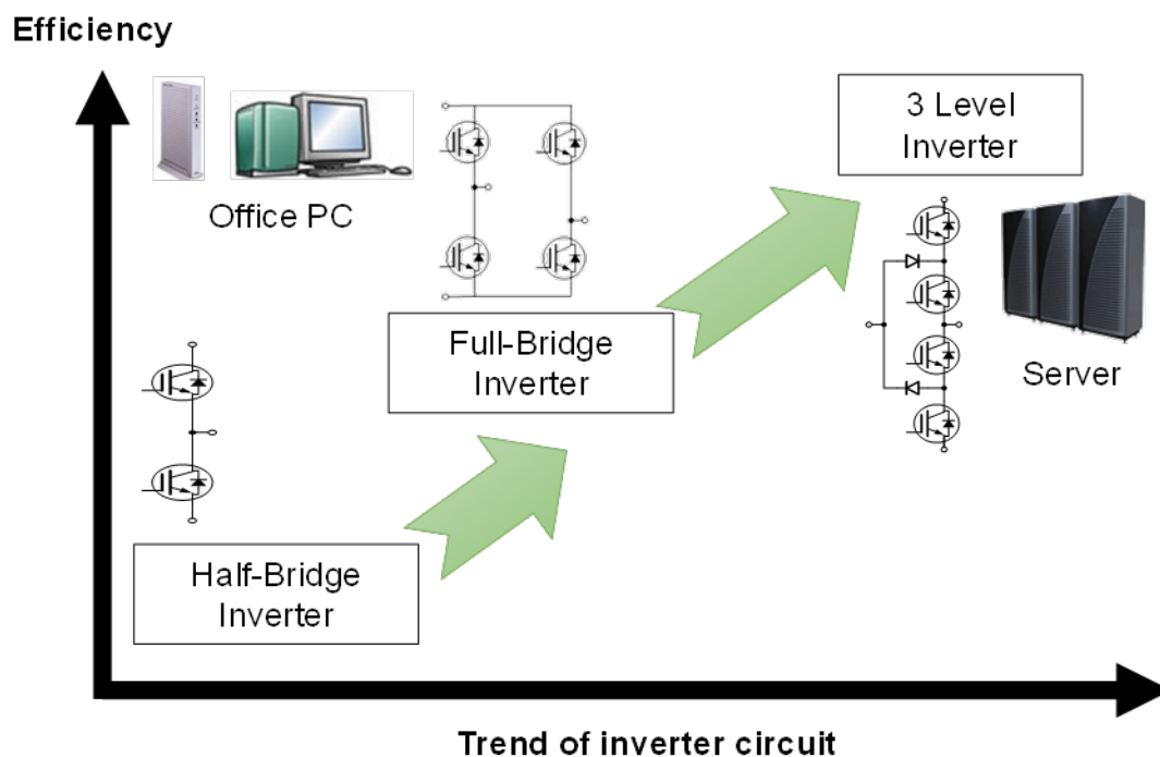
Figure 1-2 Trend of Inverter Circuit
