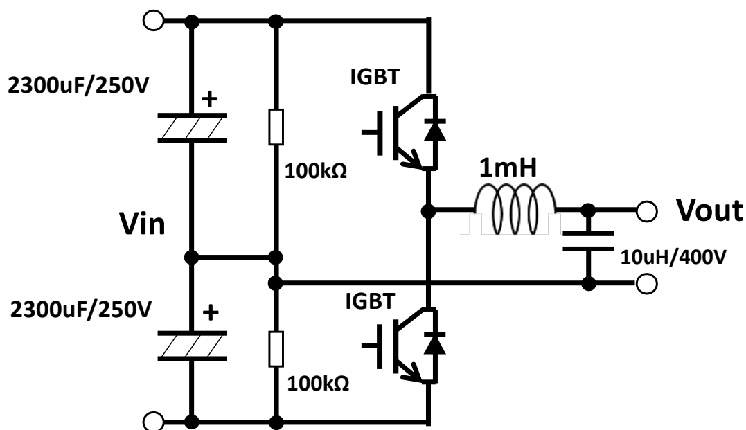
Figure 3-1 Circuit design for the Inverter
