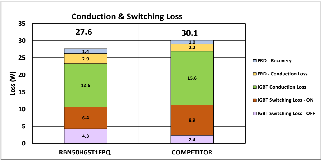
Figure 3-3 Conduction & Switching Loss Comparison
