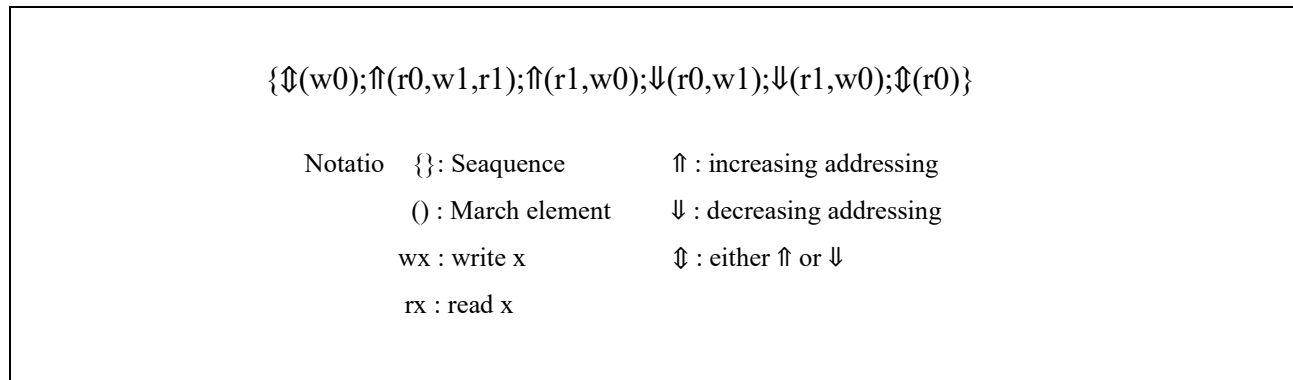
図 1-3 Extended March C- Algorithm
