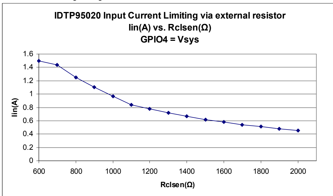
Figure 2 - Typical Input Current Limiting via external resistor, GPIO4= V_{sys}
