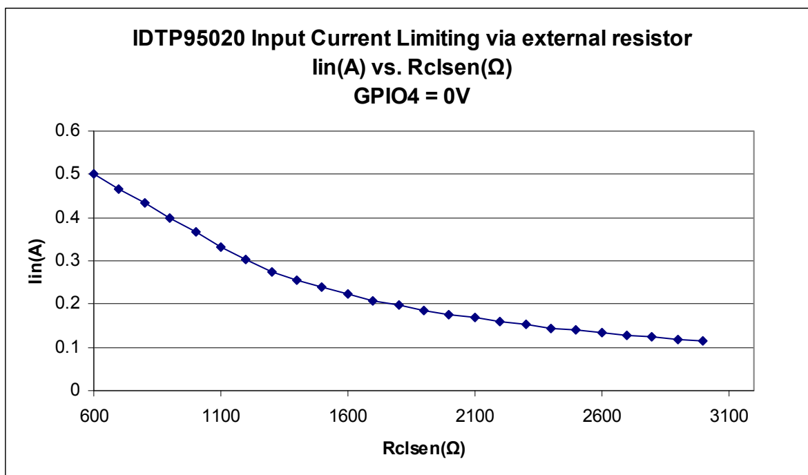
Figure 3 - Typical Input Current Limiting via external resistor, GPIO4=GND
