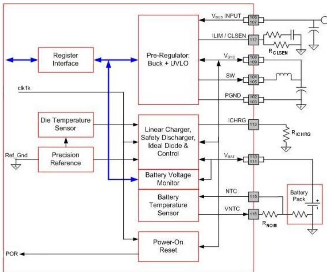
Figure 1 - Charger Block Diagram
