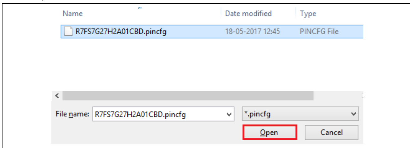
Figure 48. Synergy Configuration
