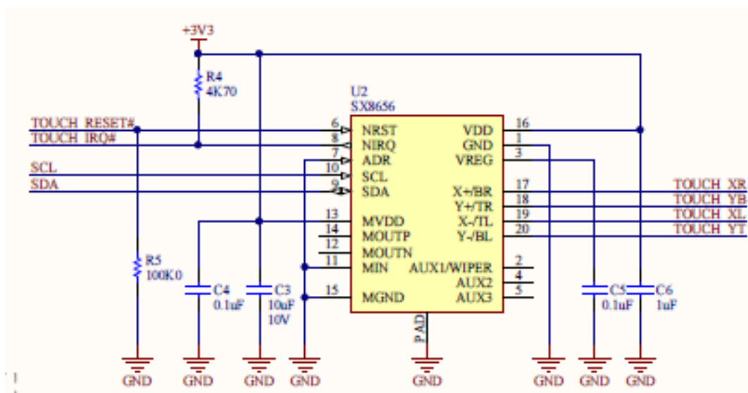
Figure 59. Touch Controller
