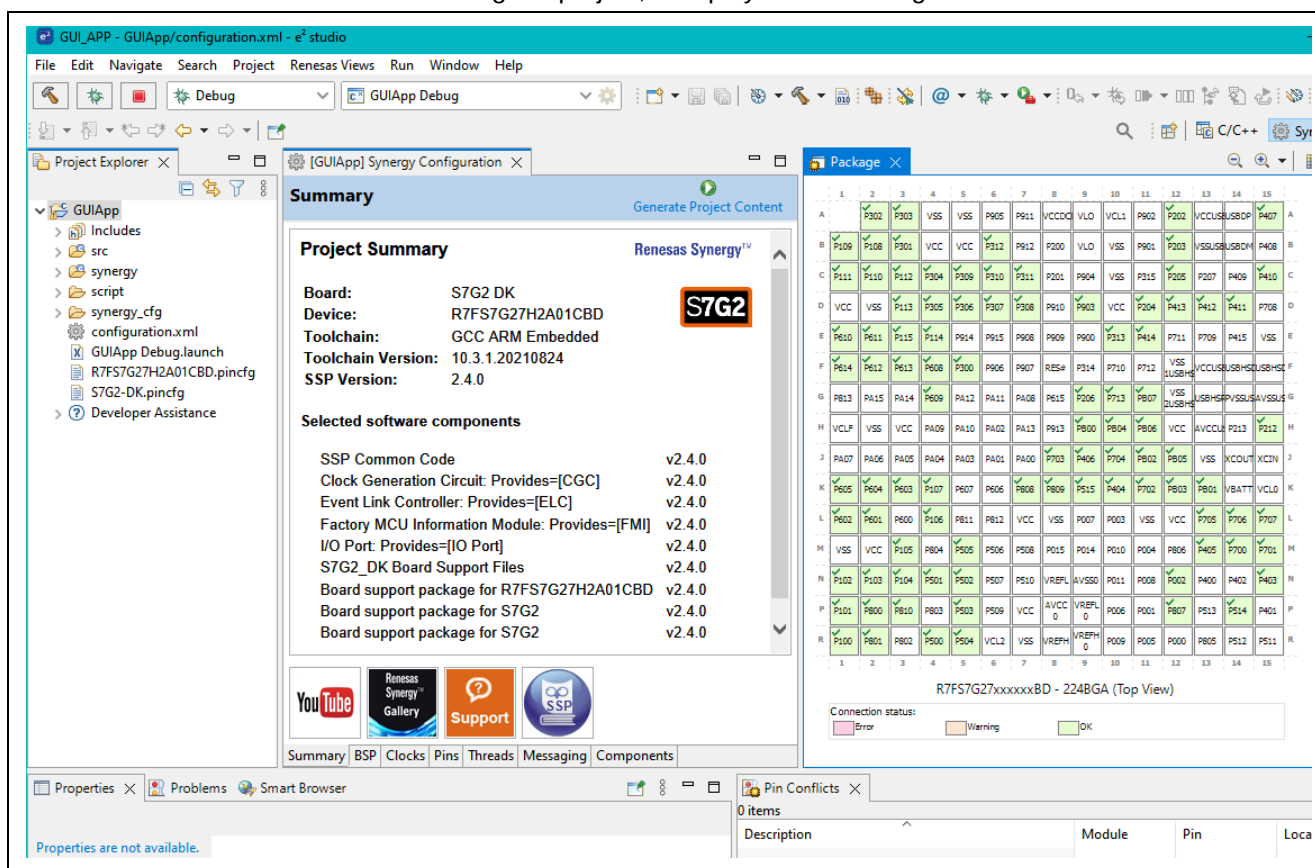
Figure 11. GUIApp Project
