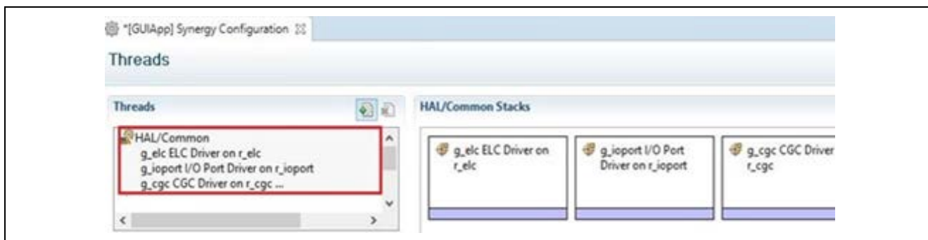
Figure 14. Threads
