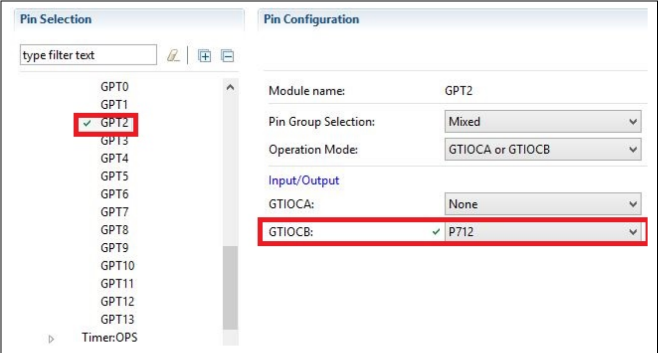
Figure 56. GPT02 Pin Configuration
