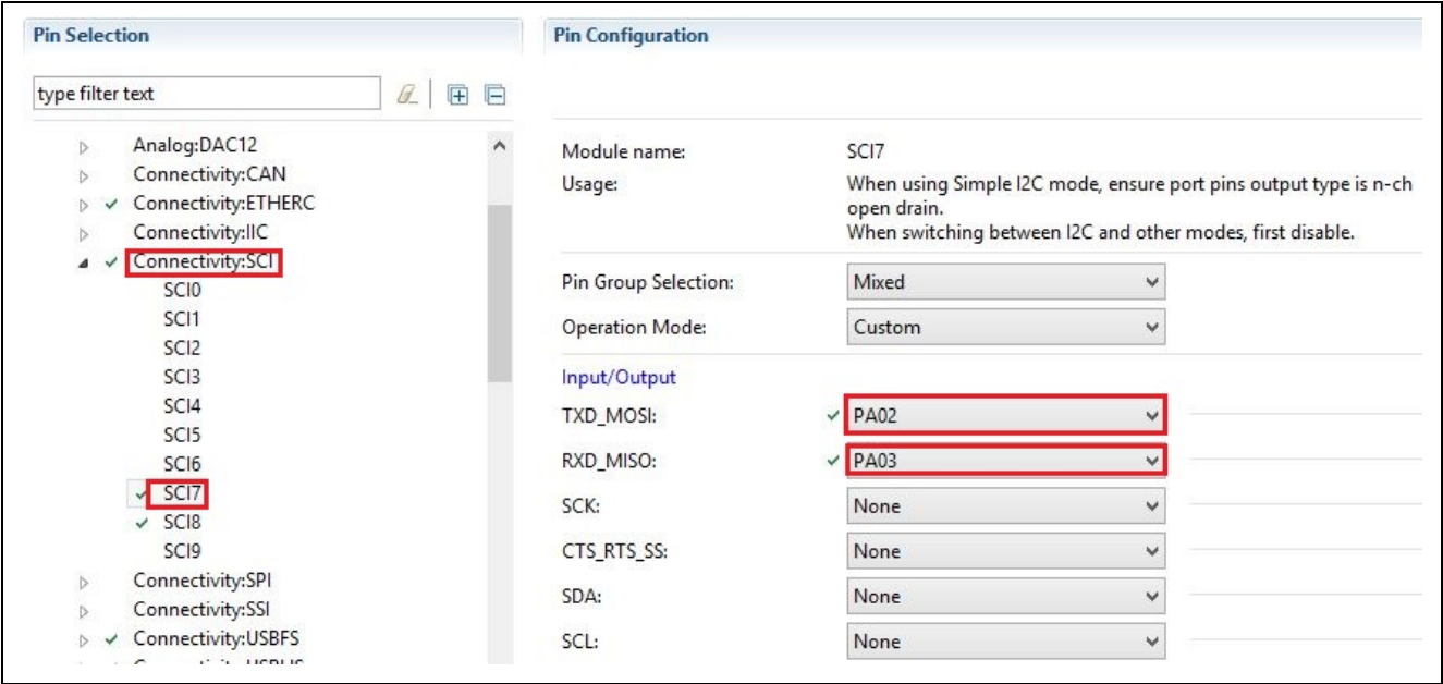
Figure 62. SCI7 Configuration
