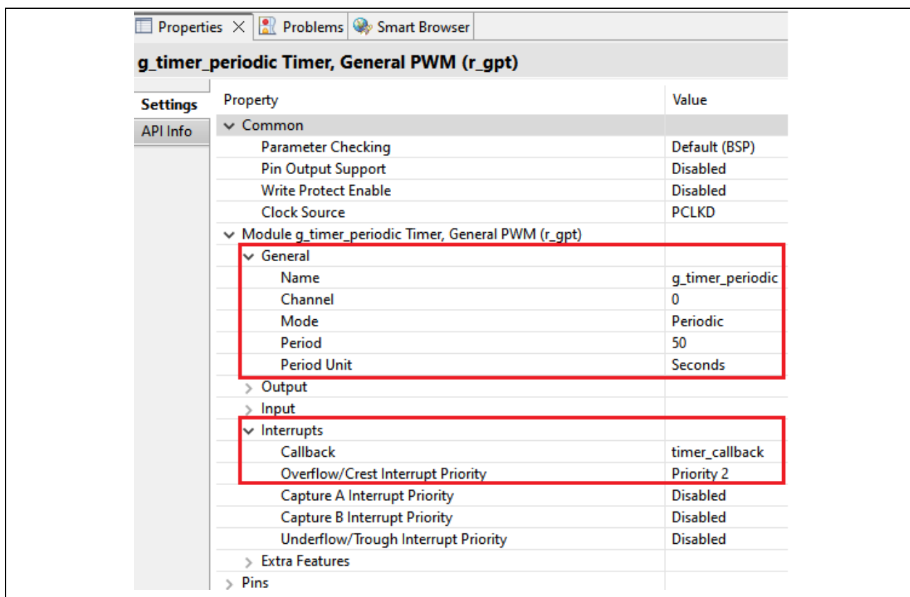
Figure 19. GPT Configuration
