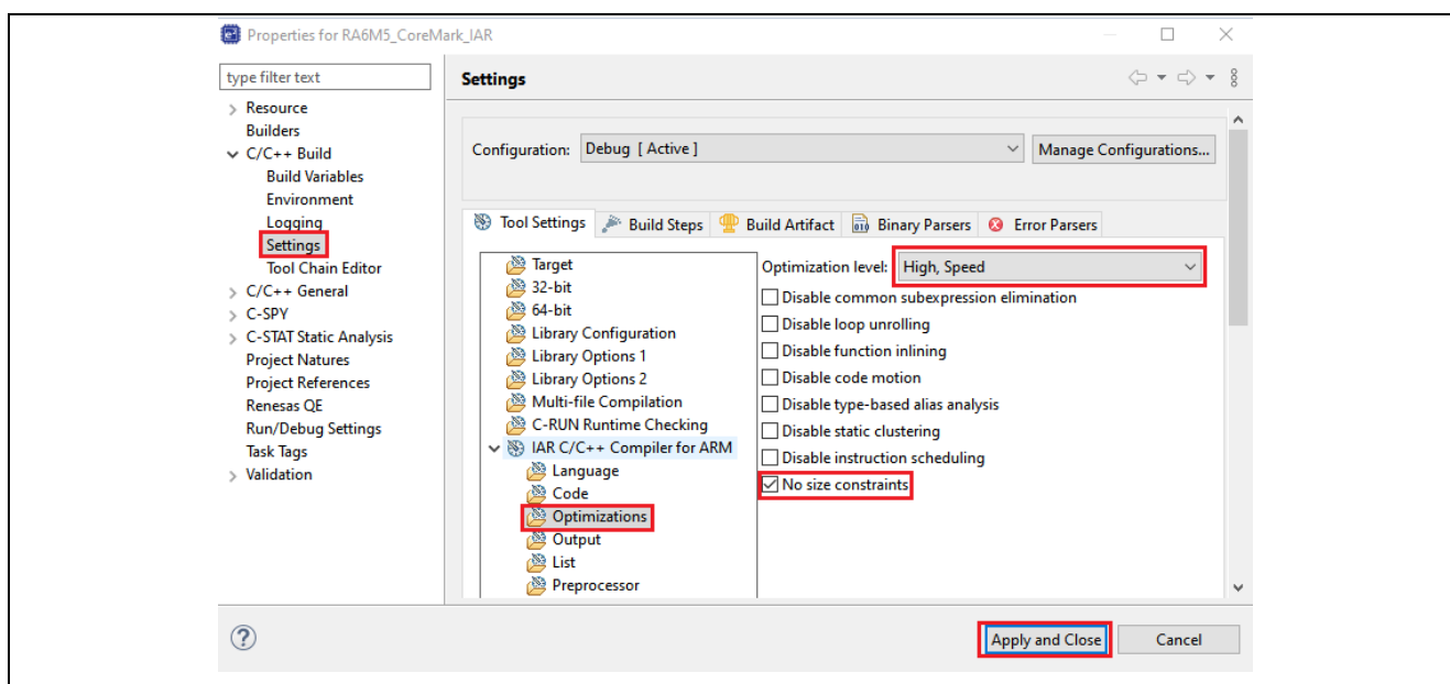
Figure 32. Optimization Setting
