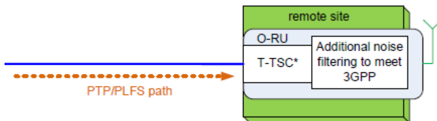
Figure 2. O-RAN S-Plane for O-RU (Figure from O-RAN.WG4.CUS.0)
