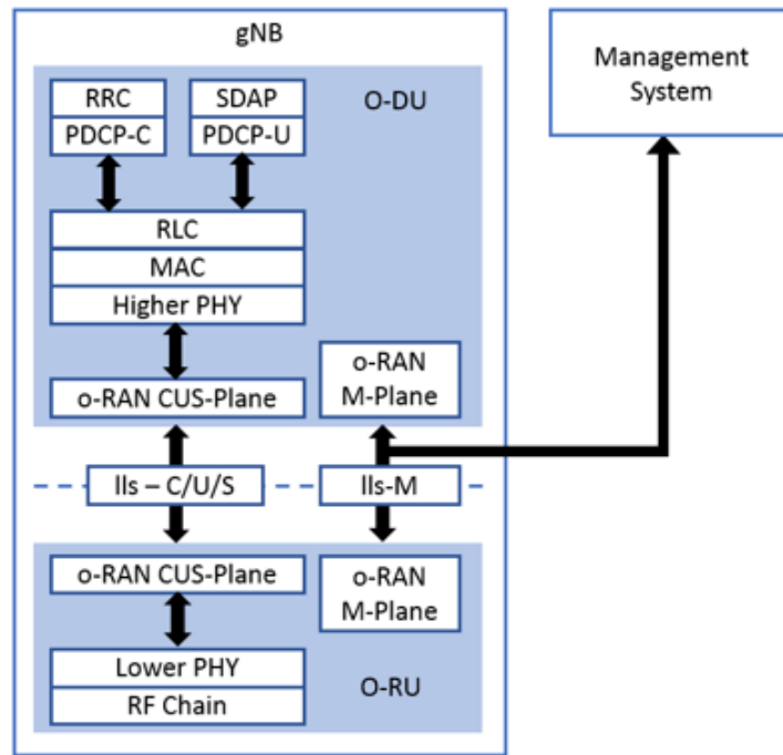
Figure 1. O-RAN Fronthaul Functional Split (Figure from O-RAN.WG4.TS.MP.0)
