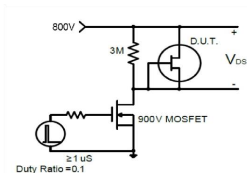
Figure 5. Spike voltage test circuit
