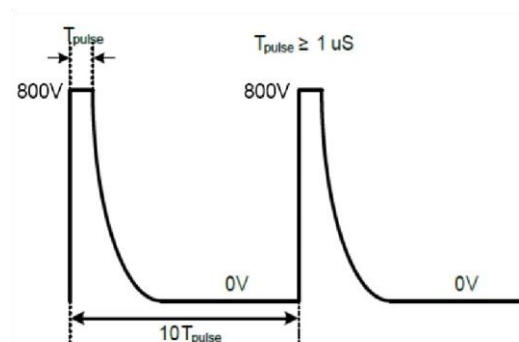
Figure 6. Spike voltage waveform
