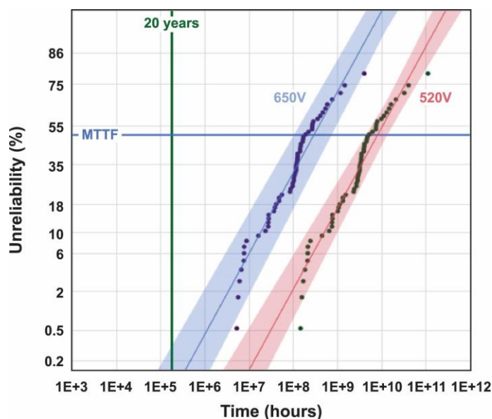
Figure 4. “Use-plots” based on voltage-accelerated testing showing all failed devices during HVOS testing at 82°C for the reciprocal field TDDb model. 99% confidence limits shown, T_j = 82^\circ\text{C} , TDDb inverse voltage model (Smith, 2015)
