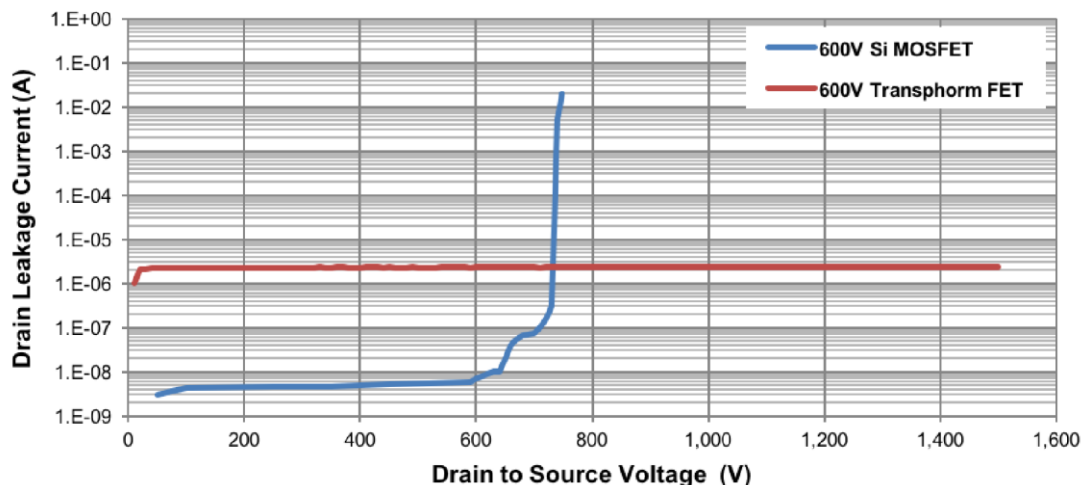
Figure 3. Off-state drain V-I characteristic - Si MOSFET vs Renesas FET
