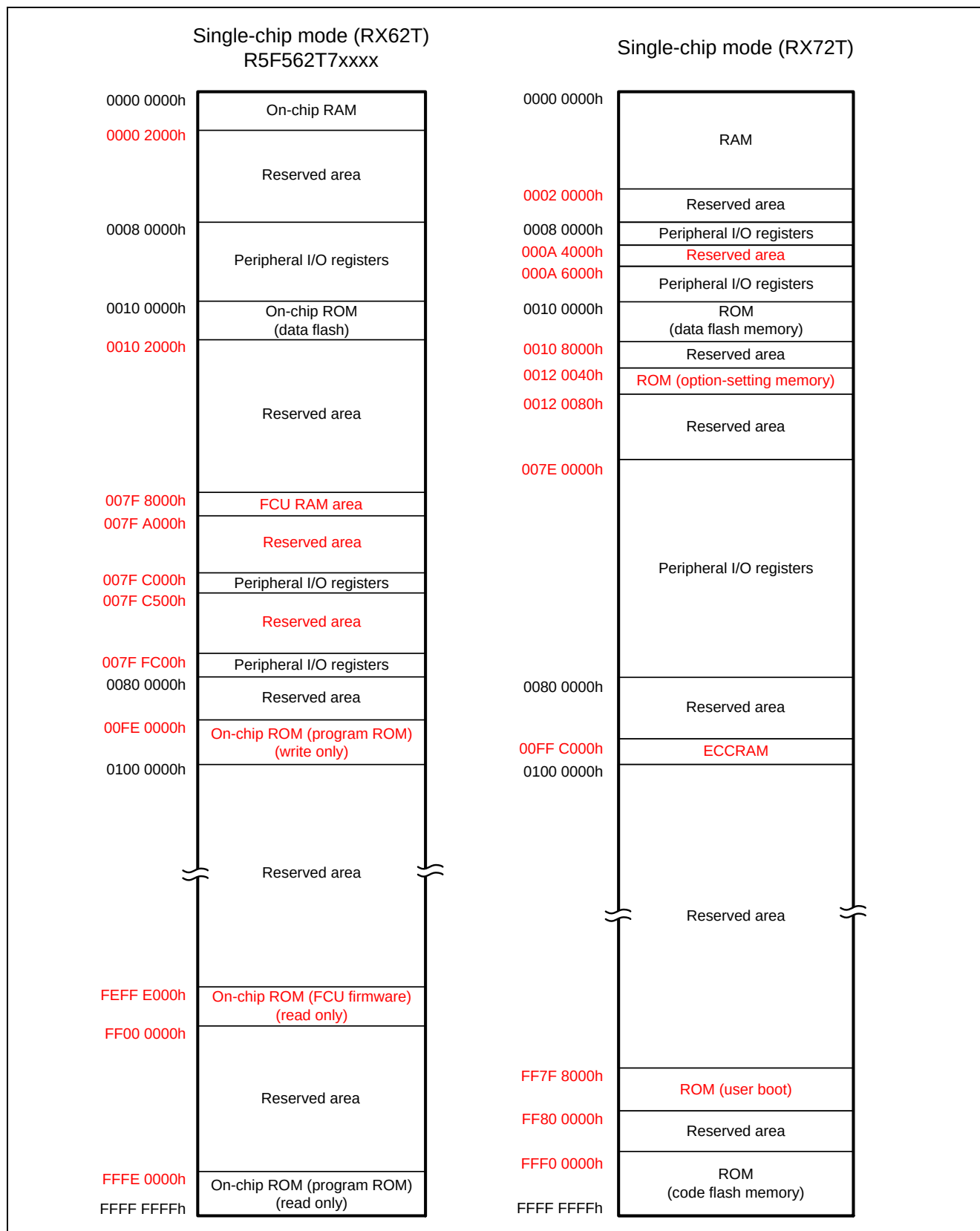
Figure 2.2 Comparative Memory Map of Single-Chip Mode (RX62T: R5F562T7xxxx)
