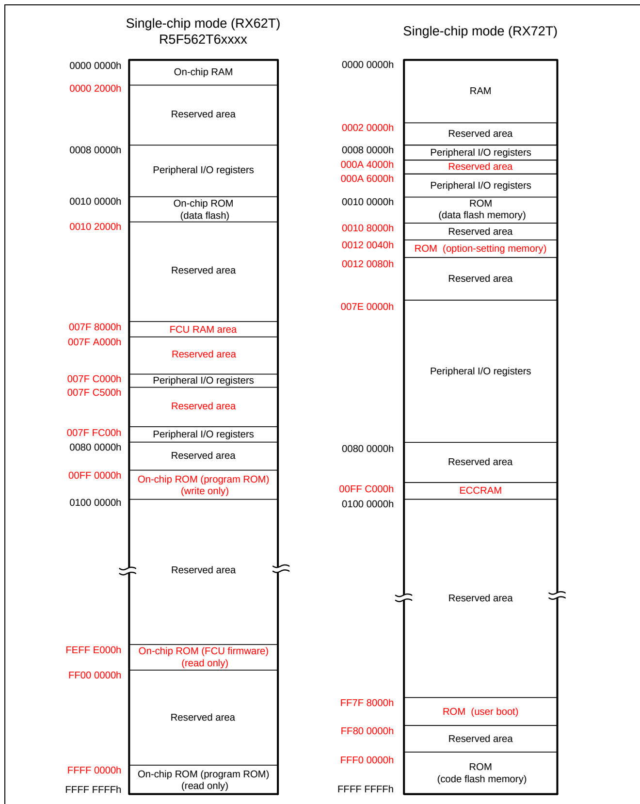
Figure 2.3 Comparative Memory Map of Single-Chip Mode (RX62T: R5F562T6xxxx)
