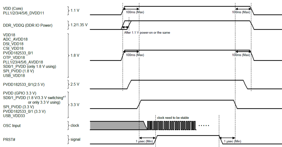
Figure 1: RZ/G2L and RZ/V2L MPU Power On/Off Sequence
