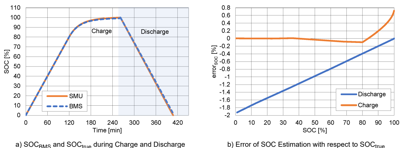
Figure 9. Cycle 3: Representative of Maximum SOC Estimation Error
