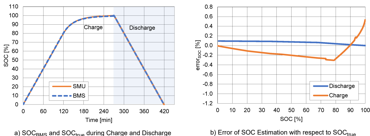
Figure 8. Cycle 2: Representative of Minimum SOC Estimation Error
