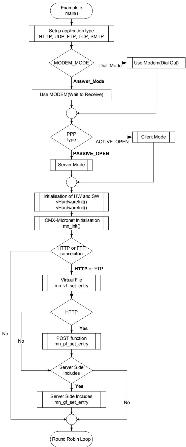
Figure 5-7 CMX-Micronet Setup Flow Diagram
