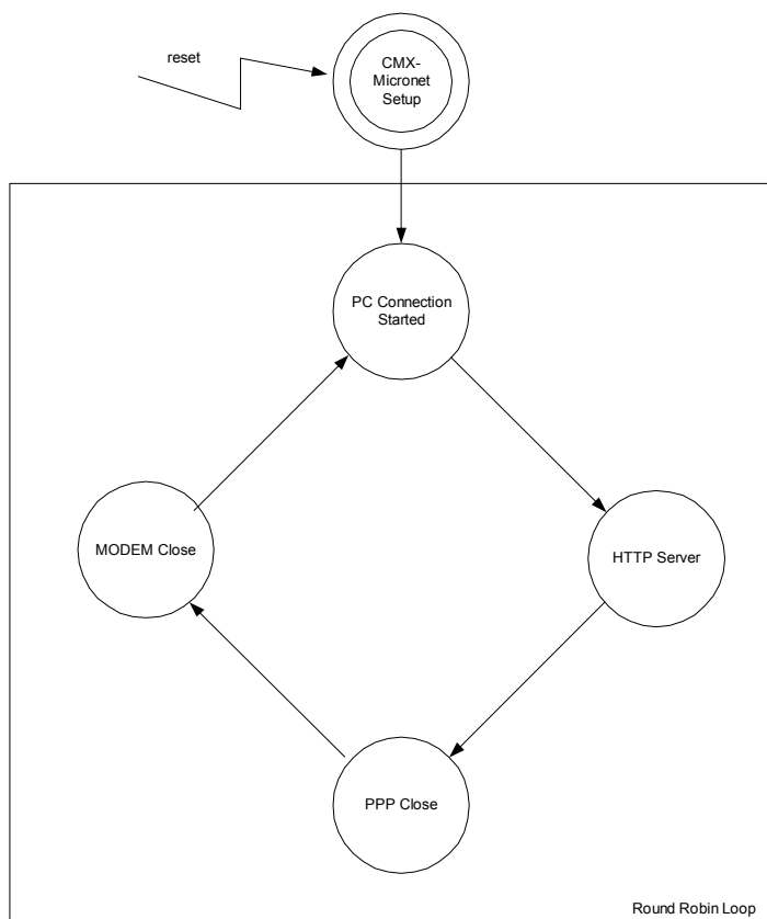
Figure 5-6 State Diagram for Example.c
