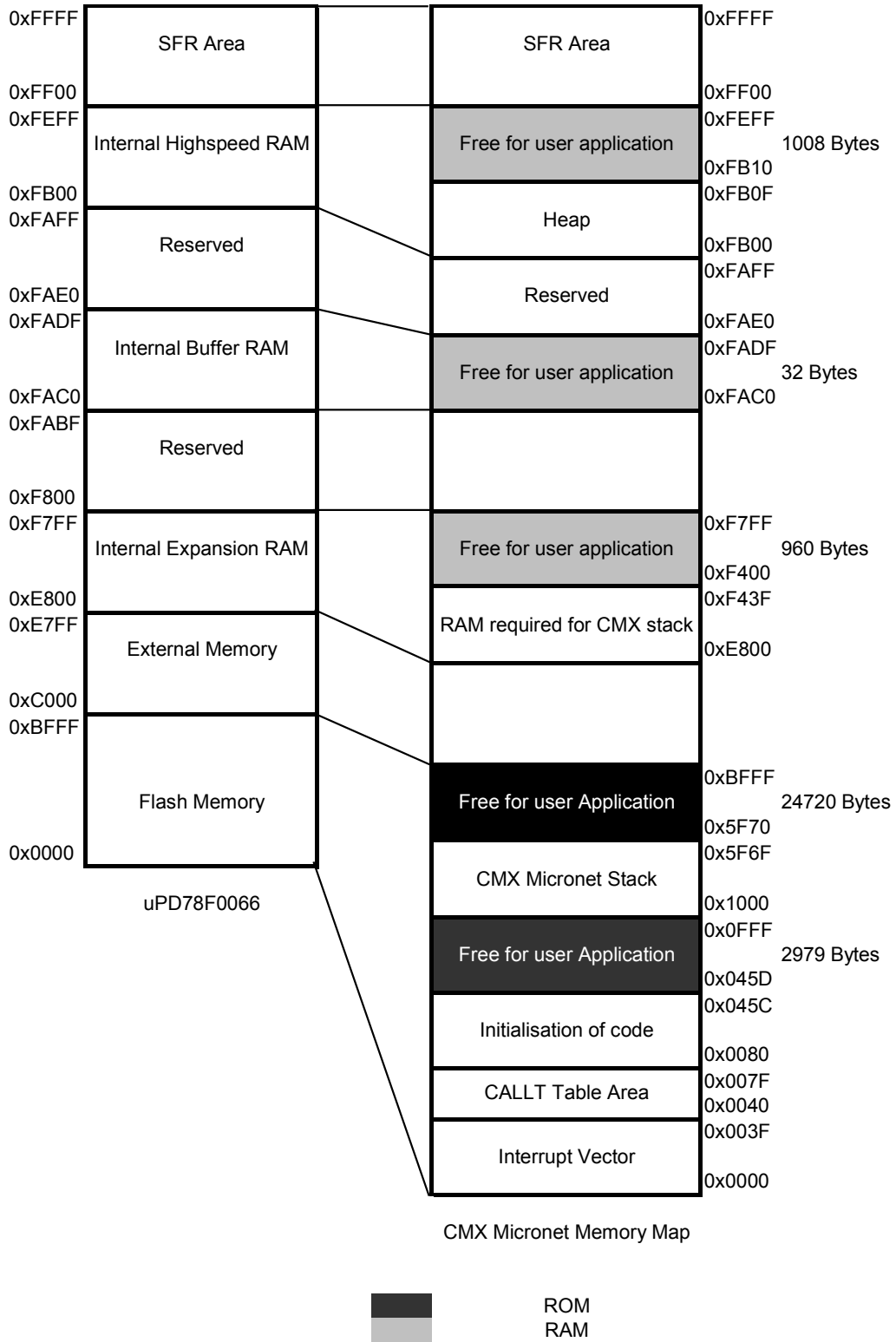
Figure 3-2 Memory Map
