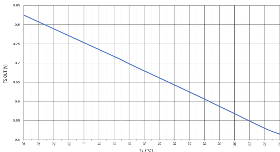
Figure 3. TS Output vs. Temperature, V_{DD} = 1.71\text{ V to }3.6\text{ V}
