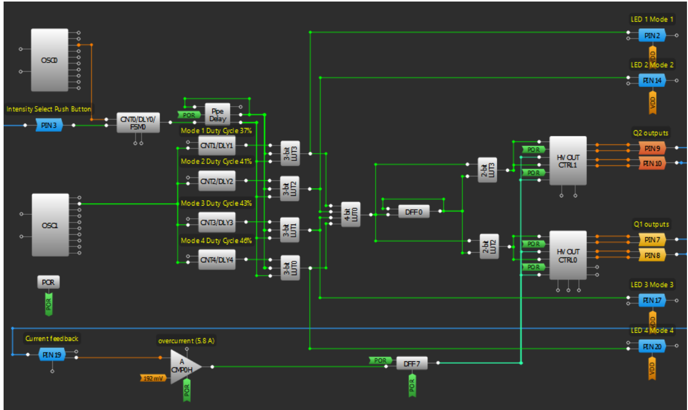
Figure 3: GreenPAK Design
