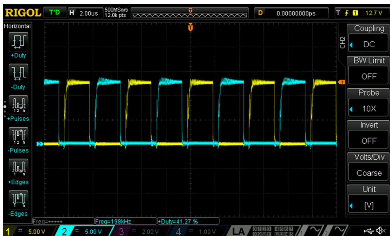
Figure 6: Mode 2 Duty cycle ~ 41%
