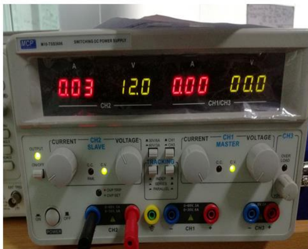
Figure 18: 12V Supply and Hardware Configuration for a Single-Phase Inverter
