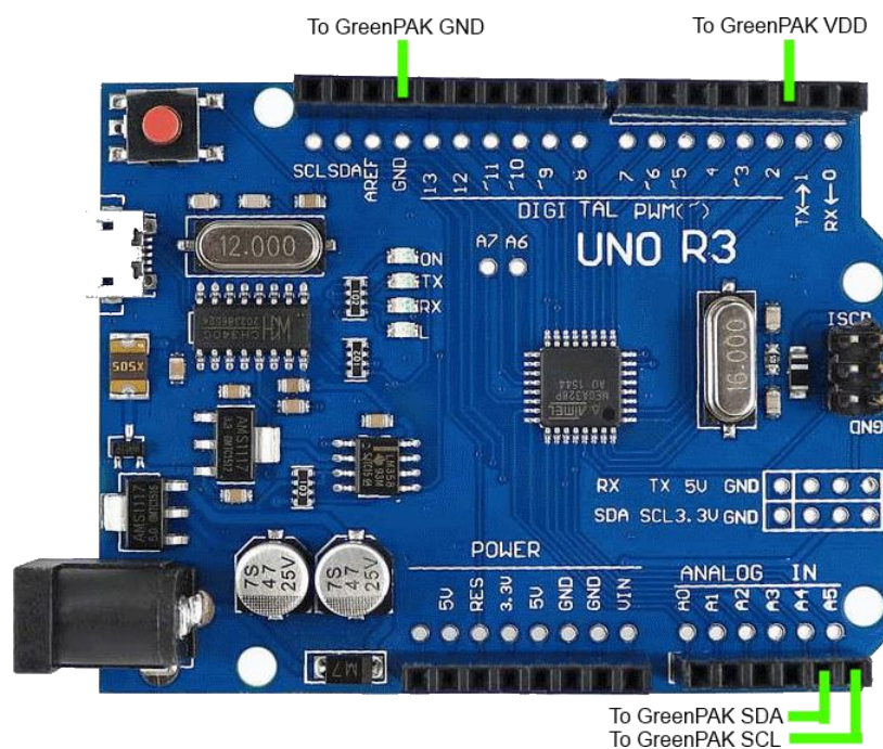
Figure 1. Arduino Connections
