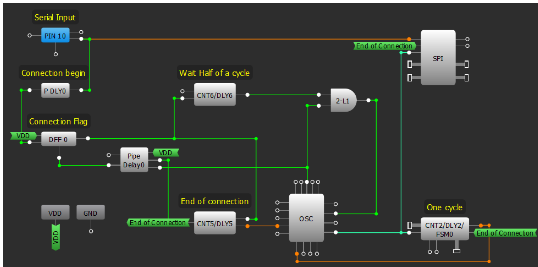
Figure 14: Serial to Parallel Converter (Matrix 0)
