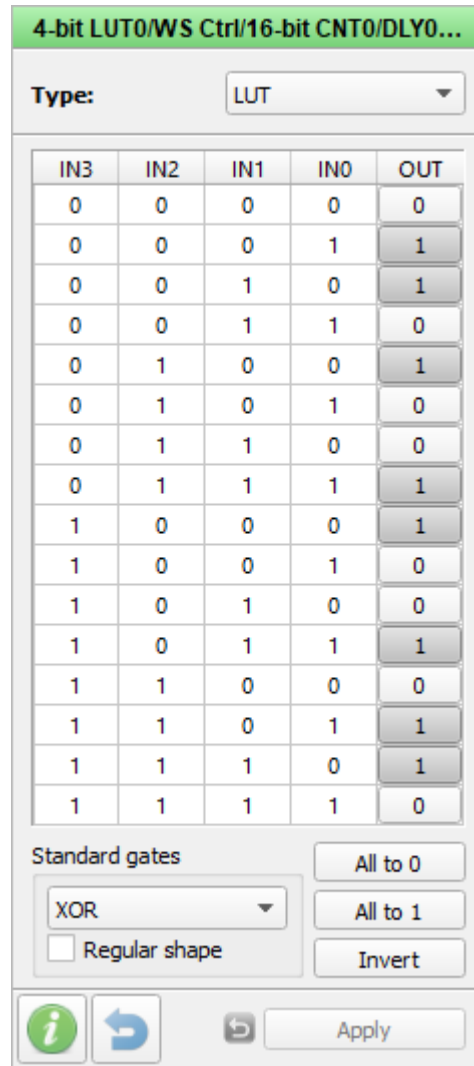
Figure 8: XOR Processor
