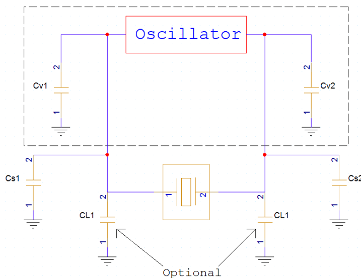
Figure 1. Crystal Capacitance
