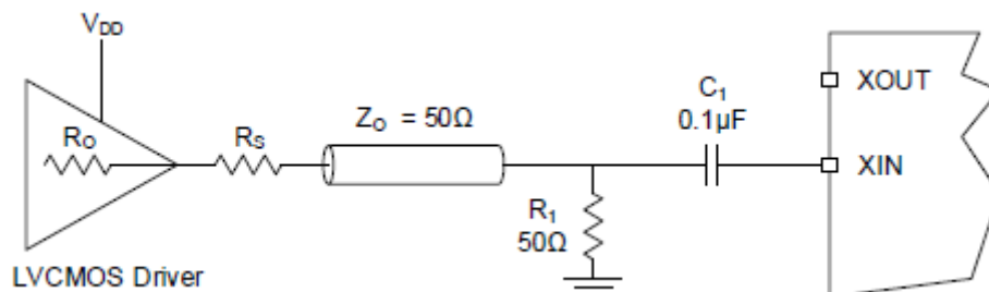
Figure 3. LVCMOS Driver to Crystal Input Interface
