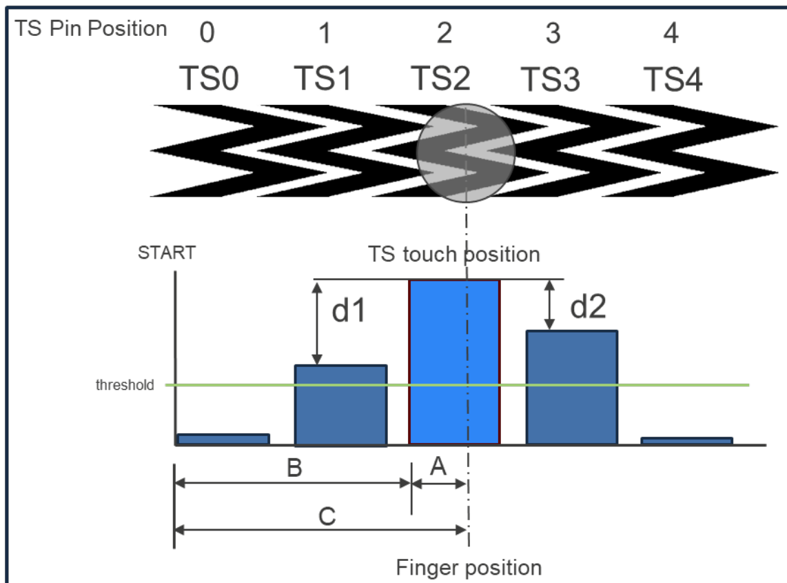
Figure 3-14 Judgement for Slider
