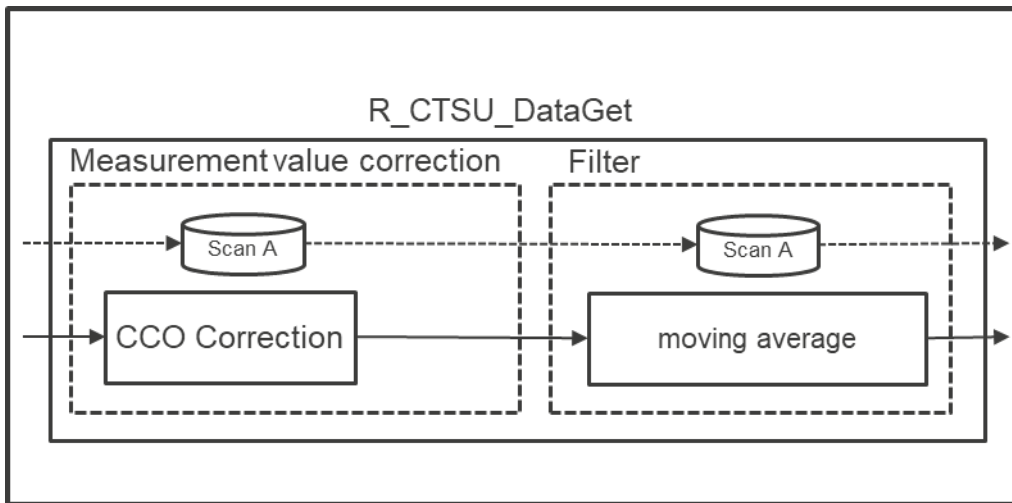
Figure 3-2 Measurement value processing in CTSU1
