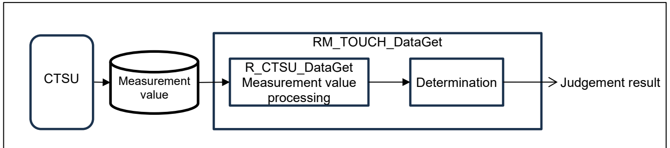
Figure 3-1 Touch judgement process
