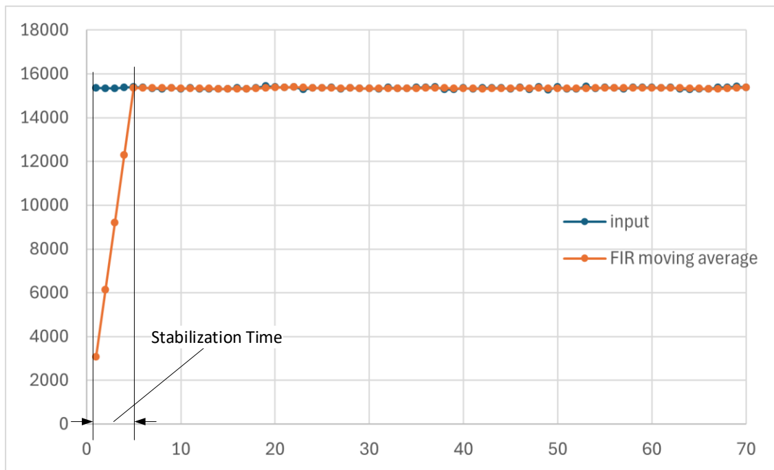
Figure 3-4 Filter Stabilization Time (FIR moving-average filter)
