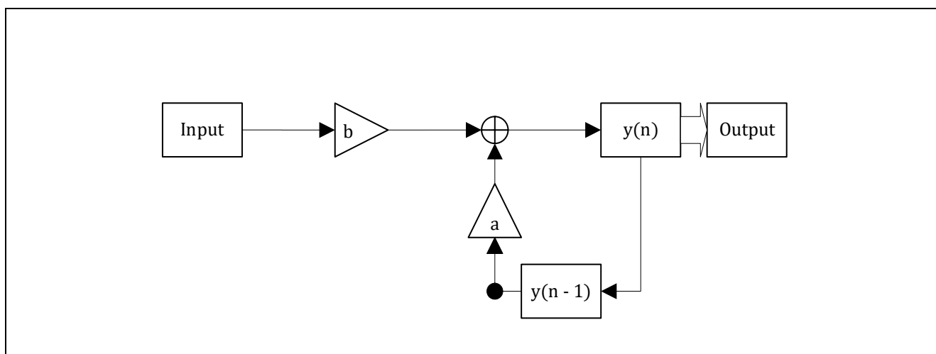
Figure 5-5 Single-pole IIR Filter Processing
