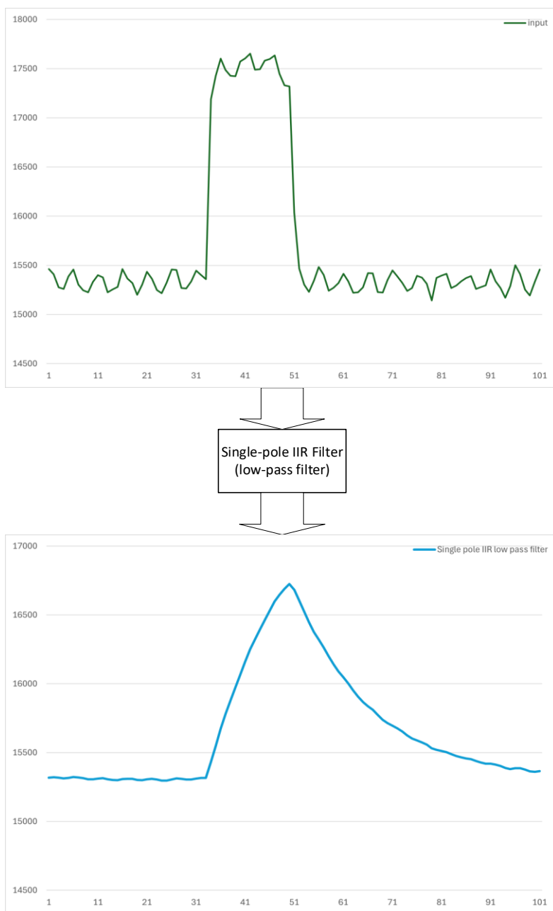
Figure 5-1 Single-pole IIR Filter Processing (low-pass filter)
