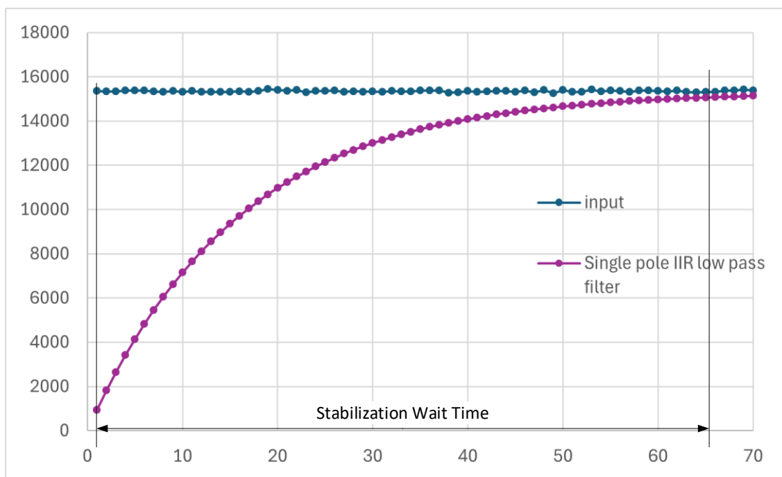
Figure 5-4 Filter Stabilization Wait Time (single-pole IIR low-pass filter)
