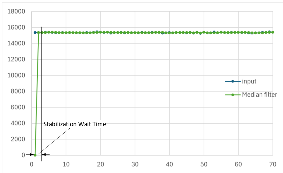
Figure 6-3 Filter Stabilization Wait Time (median)
