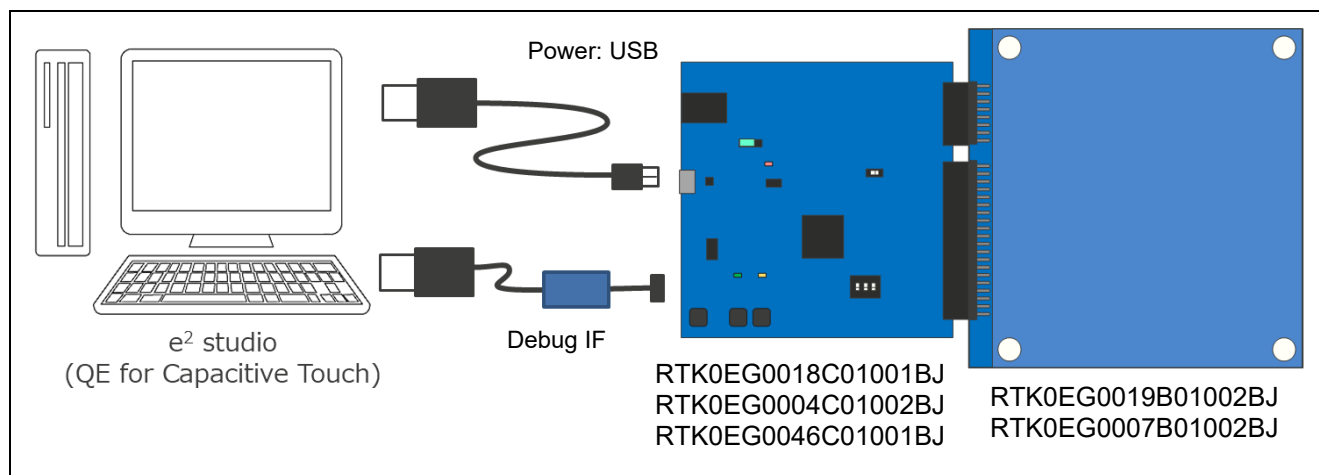
Figure 1-1 Device Connection Diagram
