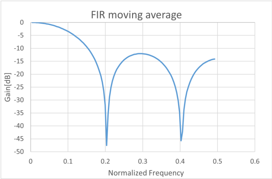
Figure 3-7 Sample FIR Filter Frequency Characteristics
