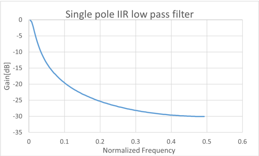
Figure 5-8 Sample Single-pole IIR Filter Frequency Characteristics
