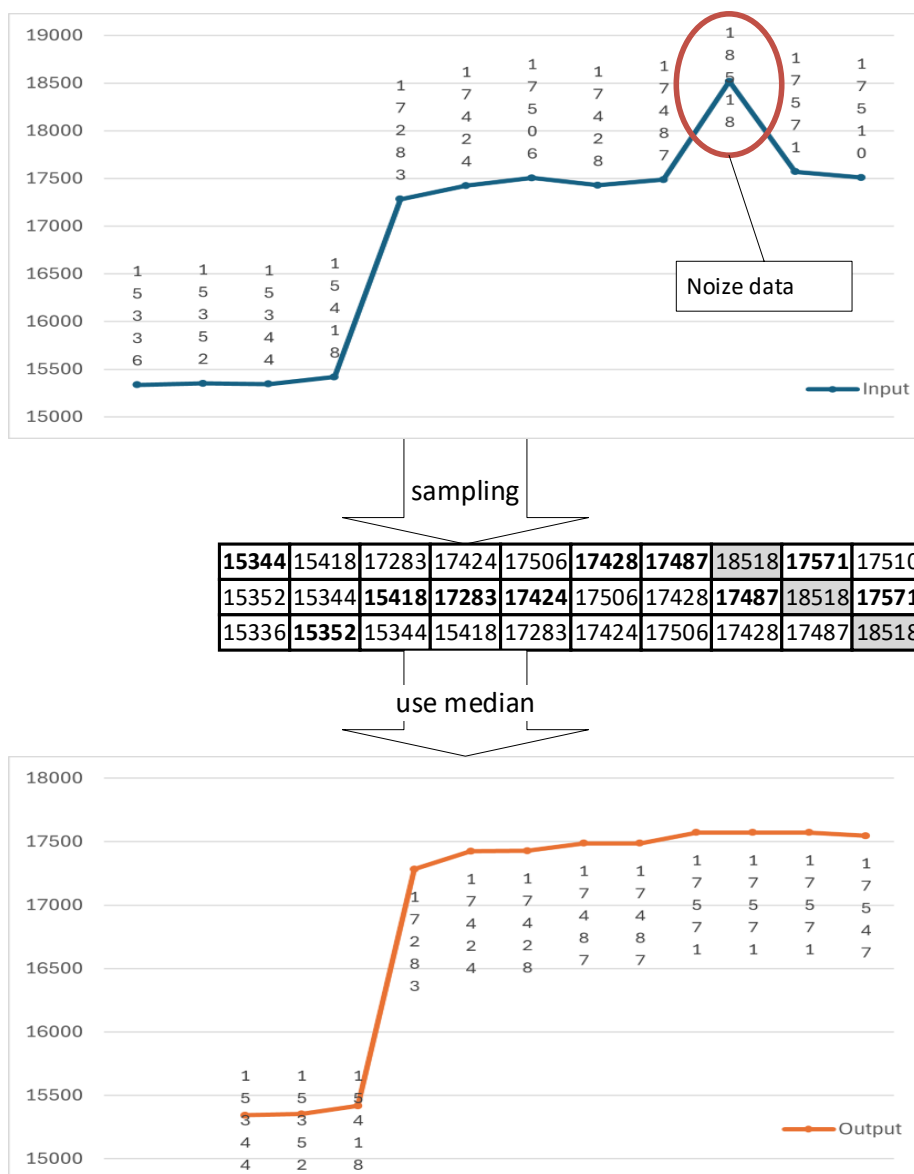
Figure 6-1 Median Filter Processing
