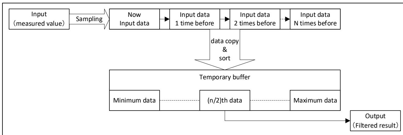
Figure 6-4 Median Filter Processing
