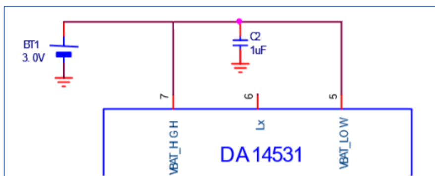
Figure 15: Bypass Configuration
