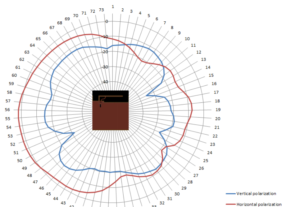
Figure 6. Radiation pattern, PCB horizontal, full-size IFA
