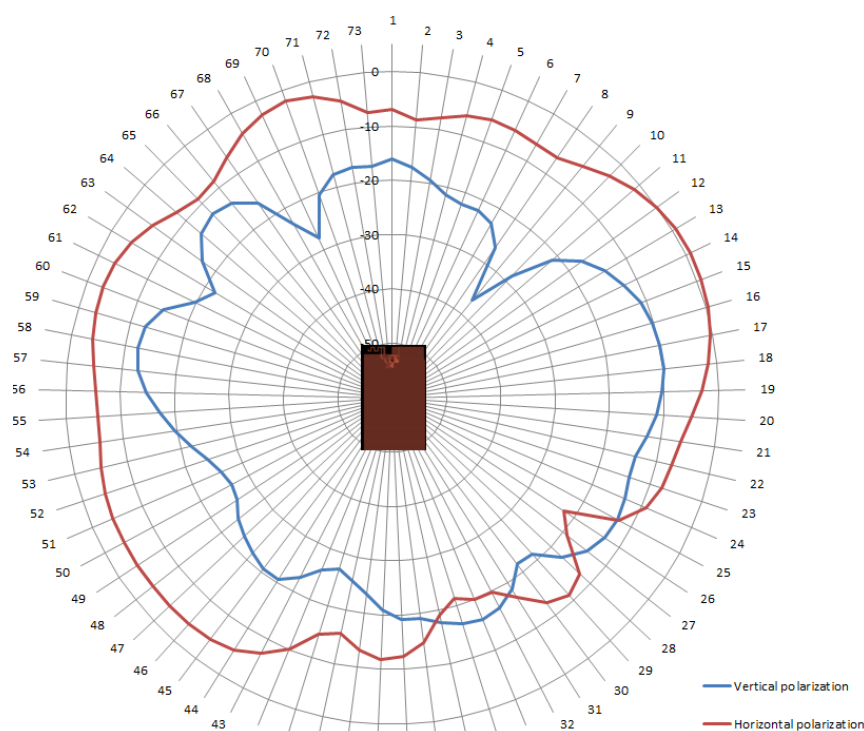
Figure 31. Radiation pattern, PCB horizontal, single layer IFA
