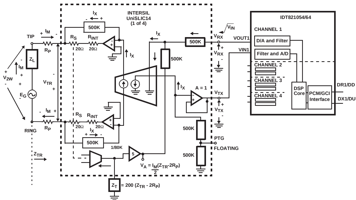
FIGURE 2. UniSLIC14 SIMPLIFIED AC TRANSMISSION CIRCUIT AND IDT821054/64
