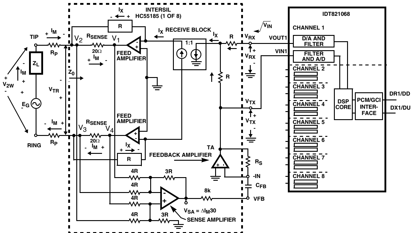
FIGURE 2. HC55185 SIMPLIFIED AC TRANSMISSION CIRCUIT AND IDT821068
