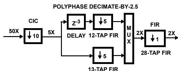
FIGURE 1. FILTER CONFIGURATION BLOCK DIAGRAM
