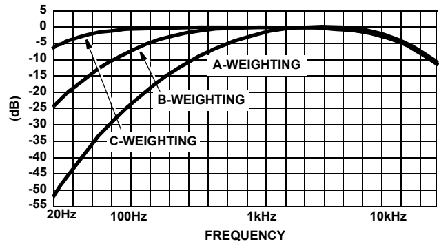
FIGURE 2. A, B, AND C WEIGHTING SYSTEMS
