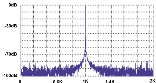
FIGURE 5. EXAMPLE OF SPECTRAL LEAKAGE
