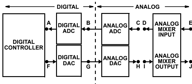
FIGURE 3. MEASUREMENT PATHS
