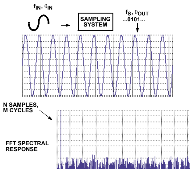
FIGURE 4. EXAMPLE OF COHERENTLY SAMPLED SYSTEM AND FFT SPECTRAL RESPONSE
