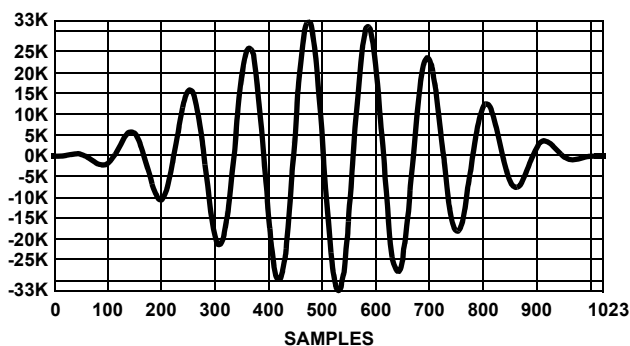
FIGURE 6. EXAMPLE OF A HANNING WINDOW
