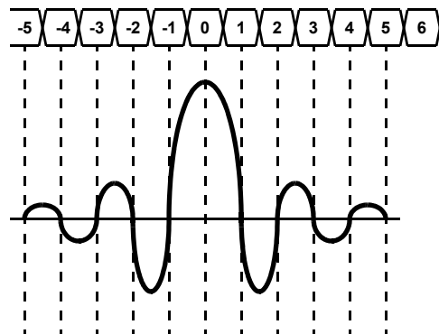
FIGURE 1. RRC FILTER CONVOLVING WITH A DATA SOURCE
