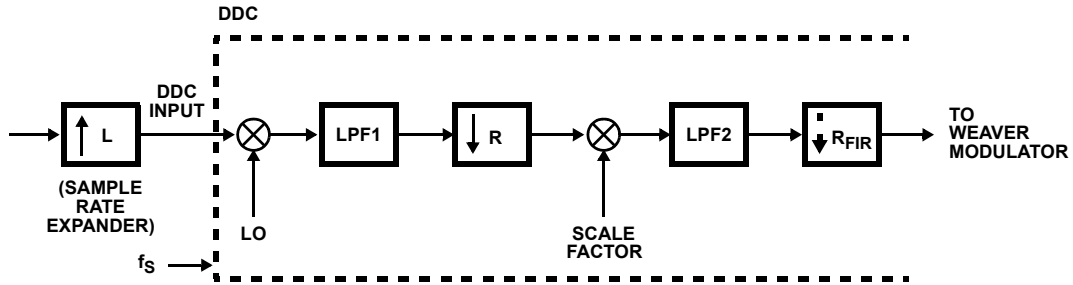
FIGURE 5. CONCEPTUAL BLOCK DIAGRAM OF ONE SIDE OF THE DDC MODULATION AND FILTER PROCESS WITH A SAMPLE RATE EXPANDER
