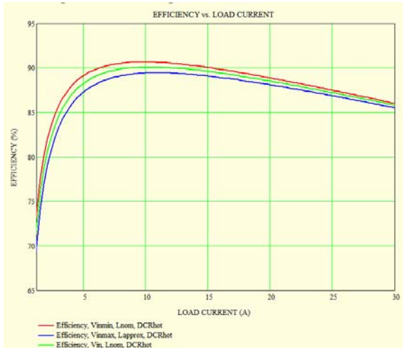
Figure 2. Predicted Efficiency
