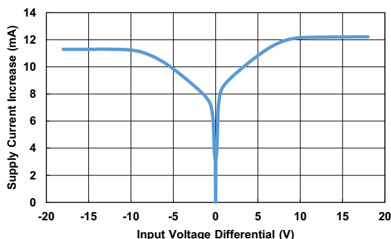
Figure 6. Simulation Input Differential Voltage vs I_{\text{SUPPLY}} Increase ( \pm 18\text{V} )
