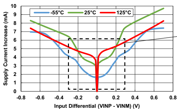
Figure 2. Typical Input Differential Voltage vs I_{\text{SUPPLY}} Increase ( \pm 18\text{V} )
