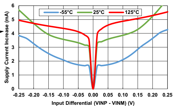
Figure 3. Typical Input Differential Voltage vs I_{\text{SUPPLY}} Increase ( \pm 18\text{V} ) (zoomed in)
