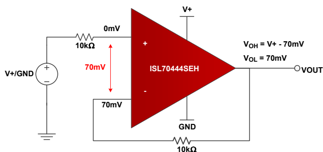
Figure 9. ISL70444SEH Configured as a Single Supply Buffer (±18V)
