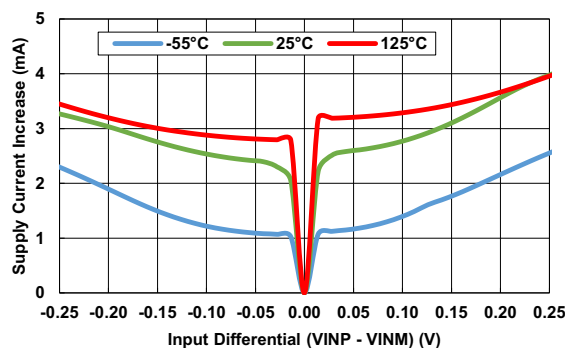
Figure 5. Typical Input Differential Voltage vs I_{\text{SUPPLY}} Increase ( \pm 2.5\text{V} ) (zoomed in)
