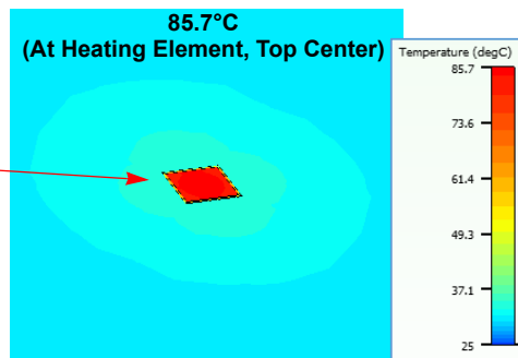
Figure 14. Zoomed In to Spot Where Most of the Power is Dissipated
