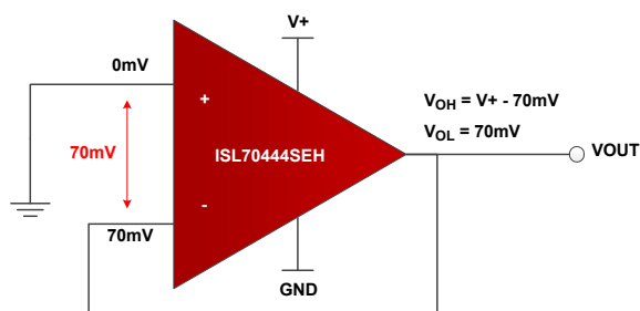
Figure 10. ISL70444SEH Unused Channel Configuration
