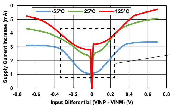
Figure 4. Typical Input Differential Voltage vs I_{\text{SUPPLY}} Increase ( \pm 2.5\text{V} )
