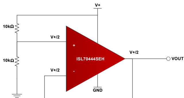
Figure 11. Recommended Configuration for Unused Op Amp Configuration to Minimize Power Dissipation
