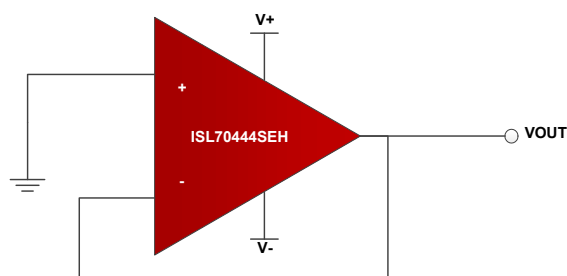
Figure 12. Recommended Configuration for Unused Op Amp Configuration for Split Supplies
