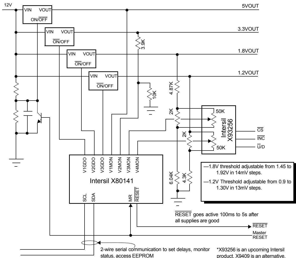
Figure 1. Dual Sequencer with Adjustable Thresholds (Block Diagram)
