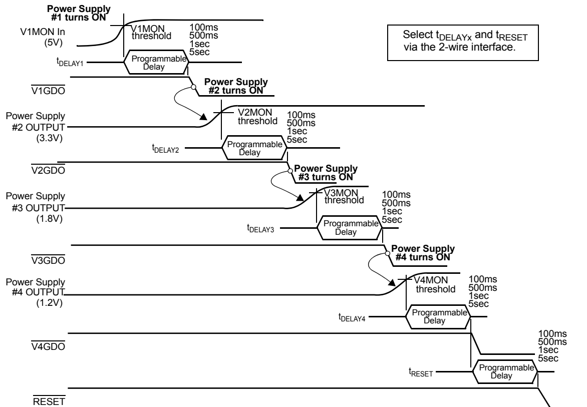
Figure 2. Sequencer Timing
