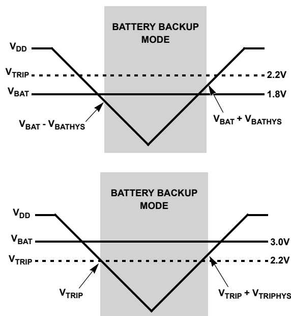
FIGURE 2. BATTERY SWITCHOVER WHEN V_{BAT} < V_{TRIP} (TOP) AND V_{BAT} > V_{TRIP} (BOTTOM)
