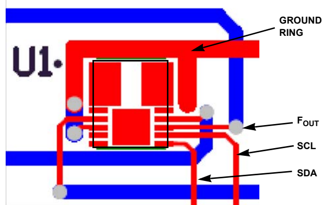
FIGURE 6. SUGGESTED LAYOUT FOR ISL12020M
