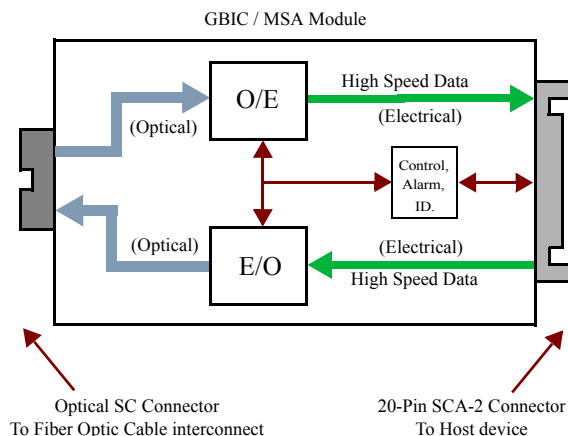
FIGURE 1. GBIC/MSA FUNCTIONAL DIAGRAM
