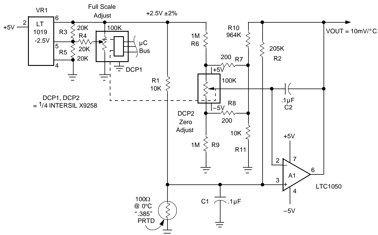
FIGURE 6. PRTD SIGNAL CONDITIONING CIRCUIT – DETAILED
