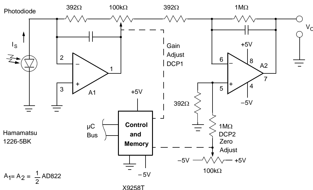
FIGURE 2. PROGRAMMABLE TRANSIMPEDANCE AMPLIFIER
