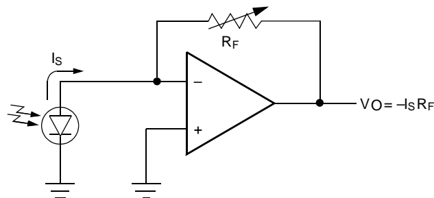
FIGURE 1. TRANSIMPEDANCE AMPLIFIER
