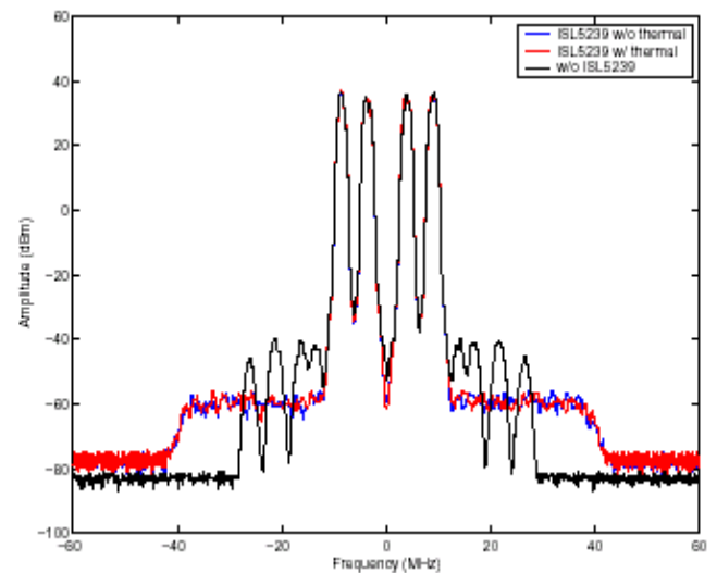
FIGURE 44J. SPECTRUM AT t = 7 ms (THERMAL COMPENSATION FOR SELF HEATING)
