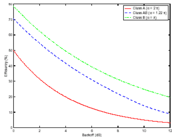
FIGURE 6. AMPLIFIER EFFICIENCY
