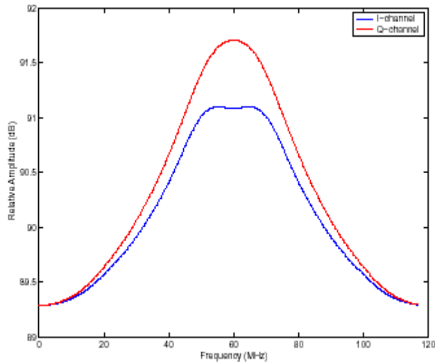
FIGURE 29A. I-CHANNEL CORRECTION FILTER RESPONSE
