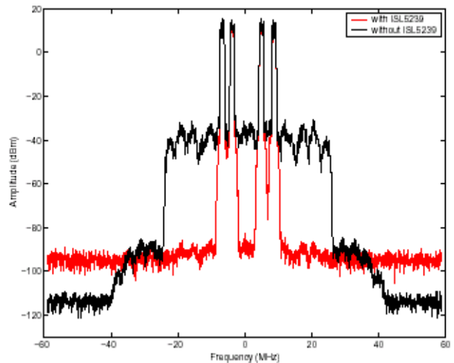
FIGURE 26B. 3% OFFSET IMBALANCE WITH CORRECTION
