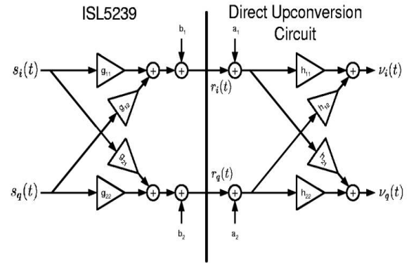
FIGURE 14. IMBALANCE COMPENSATION
