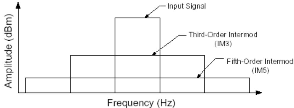
FIGURE 5. INTERMODULATION COMPONENTS
